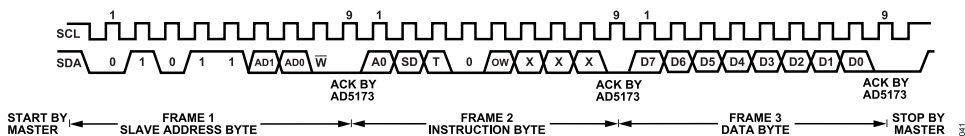
Figure 48. Writing to the RDAC Register—AD5173
