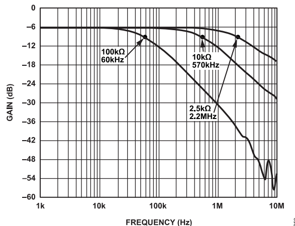
Figure 22. -3 dB Bandwidth at Code = 0x80
