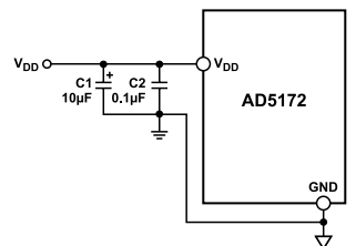
Figure 46. Power Supply Bypassing
