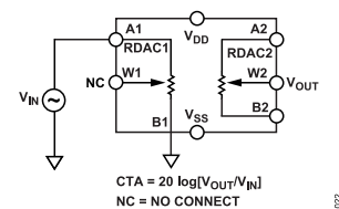
Figure 37. Analog Crosstalk
