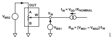
Figure 32. Wiper Resistance
