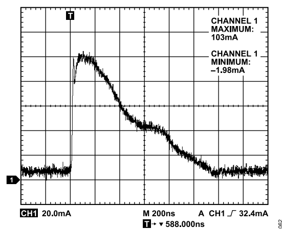
Figure 29. OTP Program Energy for Single Fuse
