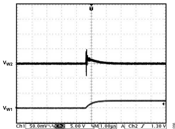
Figure 26. Analog Crosstalk
