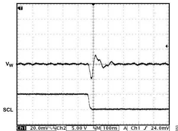
Figure 24. Digital Feedthrough
