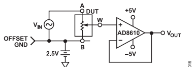
Figure 34. Test Circuit for Gain vs. Frequency
