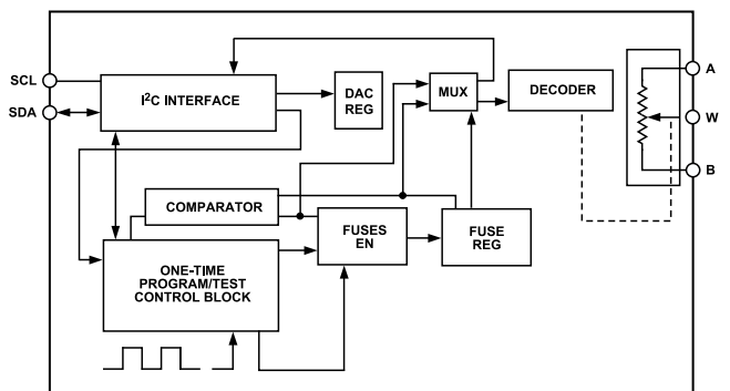
Figure 38. Detailed Functional Block Diagram
