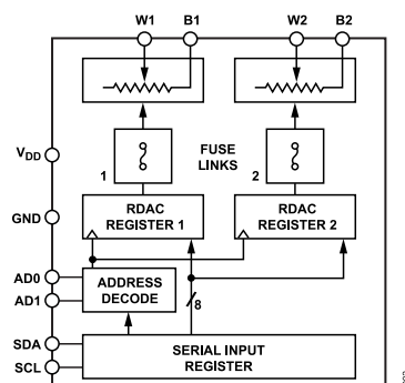
Figure 2. AD5173 Functional Block Diagram
