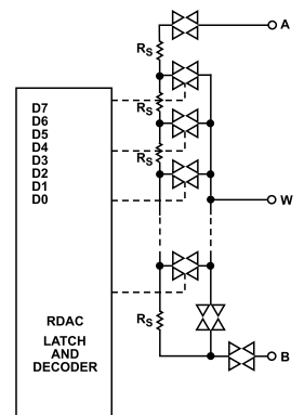
Figure 40. AD5172/AD5173 Equivalent RDAC Circuit
