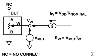
Figure 41. Wiper Resistance
