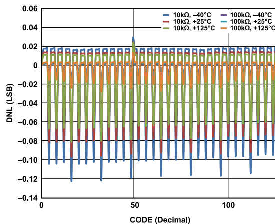
Figure 22. DNL vs. Code (AD5124)
