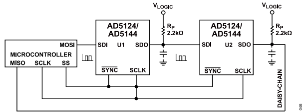
Figure 44. Daisy-Chain Configuration
