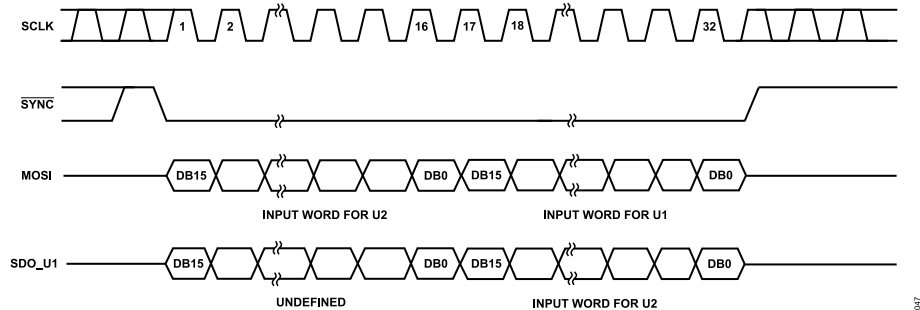
Figure 45. Daisy-Chain Diagram
