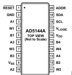
Figure 10. 20-Lead TSSOP, I²C Interface Pin Configuration (AD5144A)
