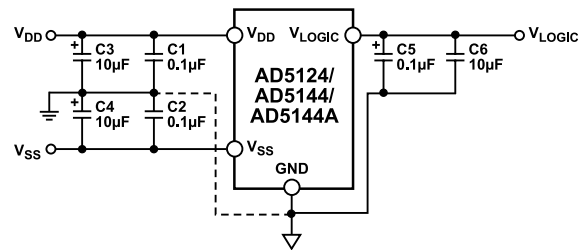
Figure 53. Power Supply Bypassing
