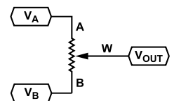
Figure 51. Potentiometer Mode Configuration
