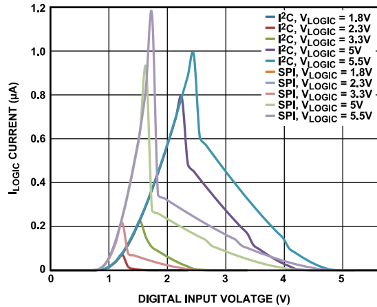
Figure 24. I_{\text{LOGIC}} Current vs. Digital Input Voltage
