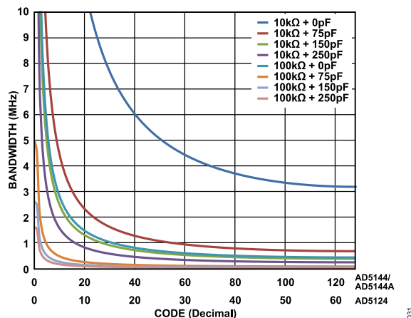
Figure 32. Maximum Bandwidth vs. Code vs. Net Capacitance
