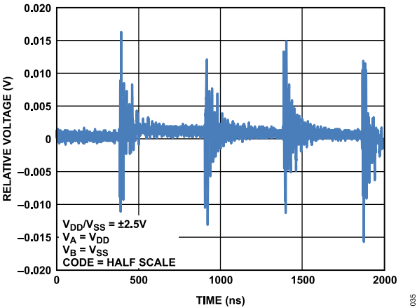
Figure 36. Digital Feedthrough
