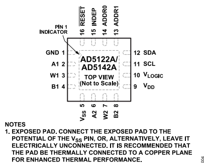
Figure 4. 16-Lead LFCSP Pin Configuration
