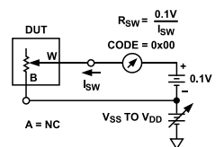
Figure 37. Incremental On Resistance
