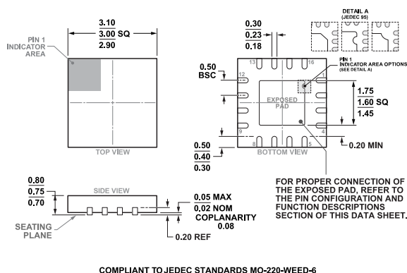
Figure 46. 16-Lead Lead Frame Chip Scale Package [LFCSP] 3 mm × 3 mm Body and 0.75 mm Package Height (CP-16-22) Dimensions shown in millimeters
