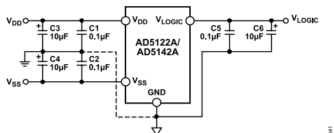
Figure 45. Power Supply Bypassing
