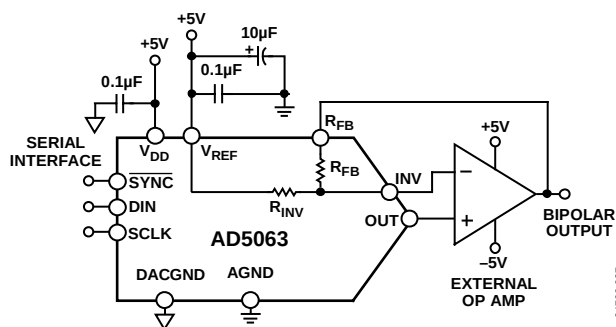
Figure 37. Bipolar Operation
