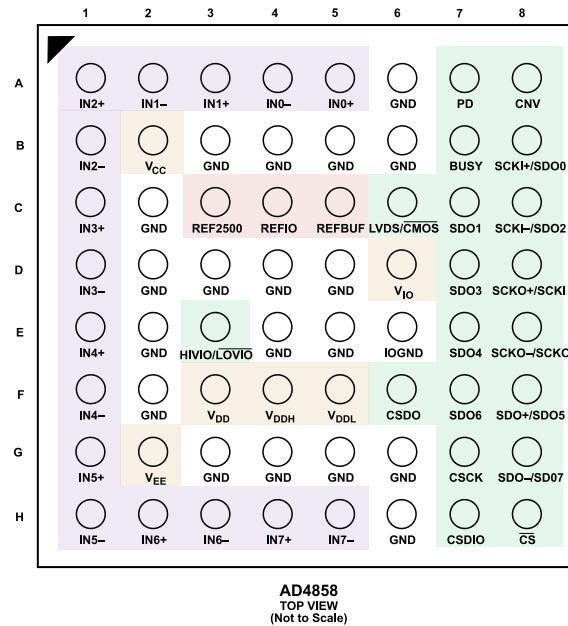
Figure 8. Pin Configuration
