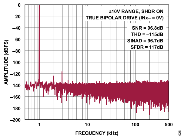
Figure 24. FFT, 1 MSPS, f_{IN} = 1 kHz, \pm 10 V Range
