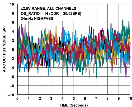
Figure 37. Low Frequency Noise over 10 seconds
