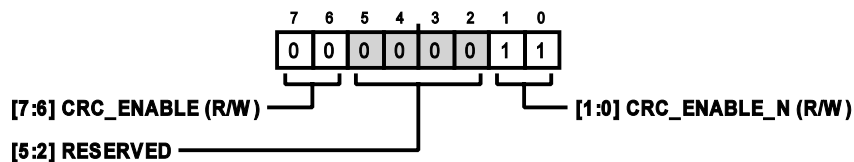
Figure 88. Address: 0x10, Reset: 0x03, Name: SPI_CONFIG_C
