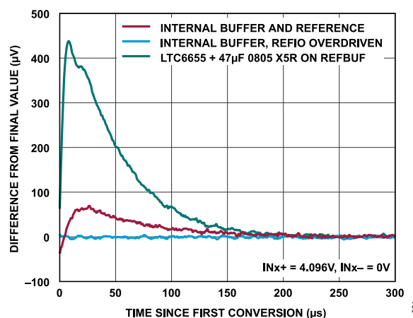
Figure 60. Burst Conversion Response of the AD4858, f_s = 1 MSPS
