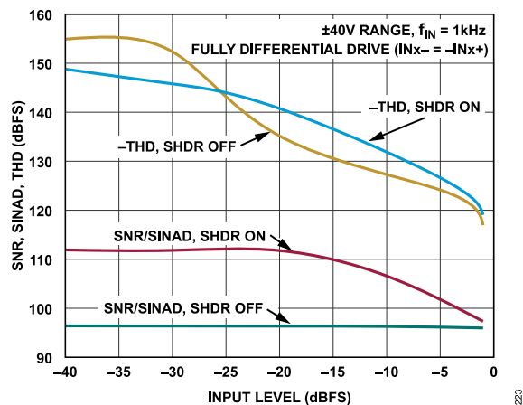
Figure 23. SNR, SINAD, and THD vs. Input Level
