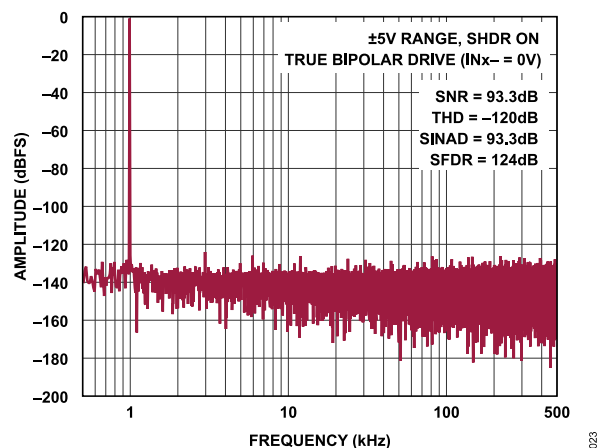
Figure 22. FFT, 1 MSPS, f_{IN} = 1 kHz, \pm 5 V Range
