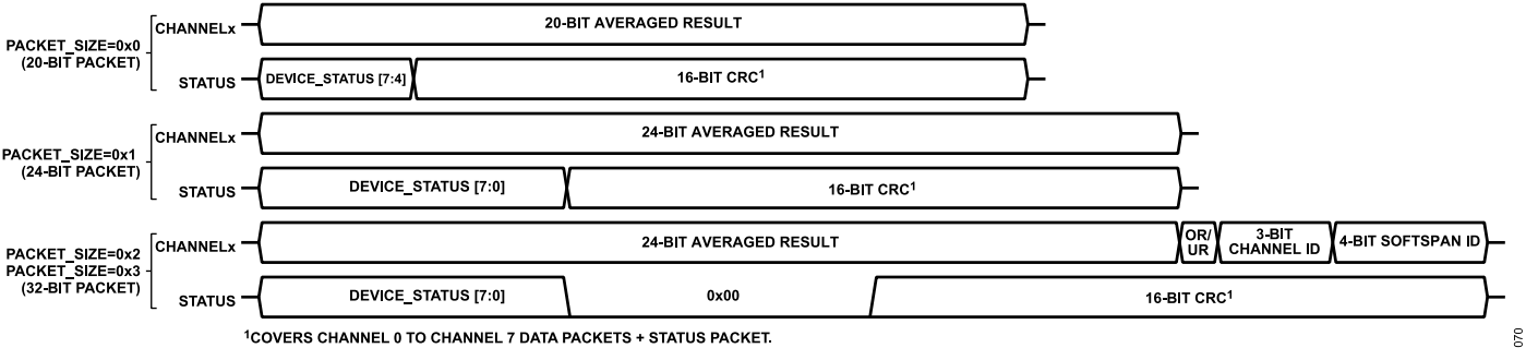
Figure 71. Channel and Status Packet Data Formats in Oversampling Mode (OS_EN = 1), Test Pattern Output is Disabled (TEST_PAT = 0)
