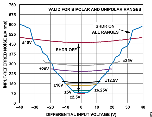
Figure 18. Input-Referred Noise vs. Differential Input Voltage
