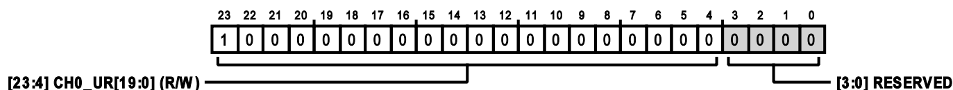
Figure 105. Address: 0x35 to Address 0x37, Reset: 0x800000, Name: CH0_UR
