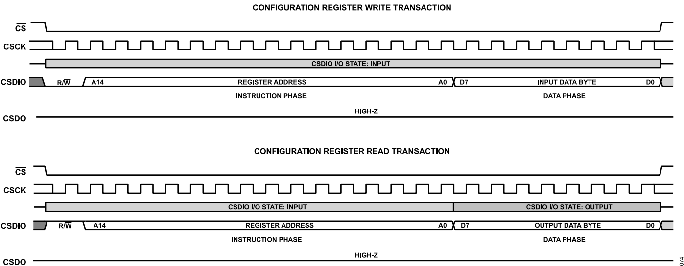
Figure 73. 3-Wire SPI Register Configuration Bus Frame
