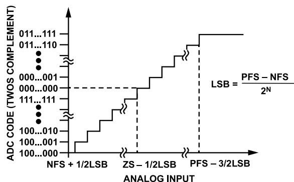
Figure 49. AD4858 Ideal Bipolar Input Transfer Function. N = 20 bits
