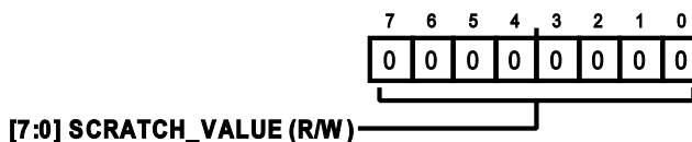
Figure 82. Address: 0x0A, Reset: 0x00, Name: SCRATCH_PAD
