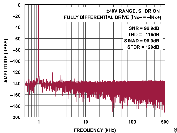
Figure 21. FFT, 1 MSPS, f_{IN} = 1 kHz, \pm 40 V Range
