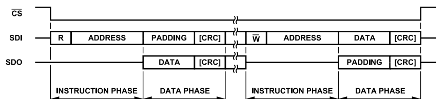
Figure 90. Single Instruction Mode SPI Frame
