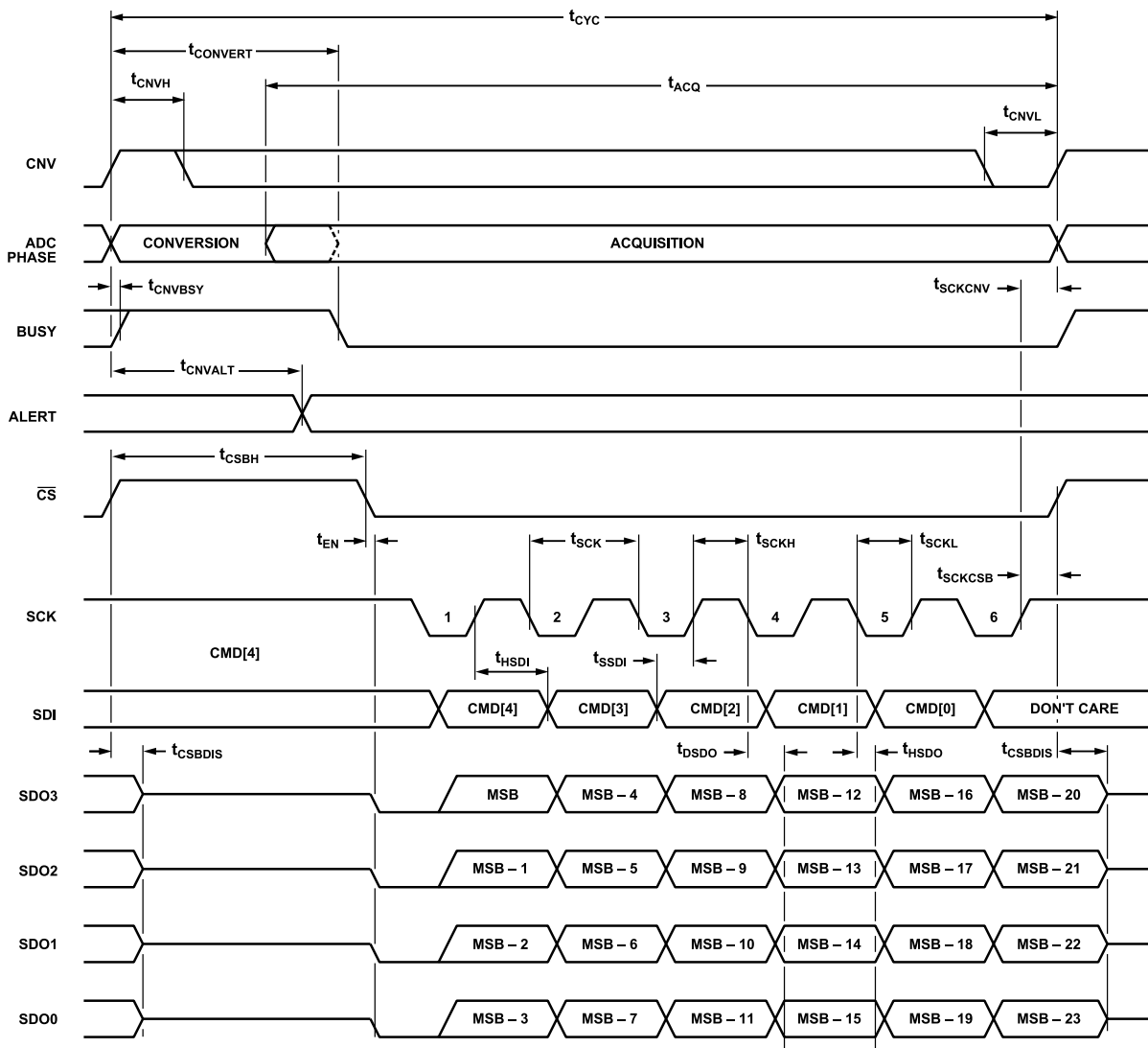
Figure 100. Conversion Mode Timing Diagram, Quad-SDO Mode, SDO\_STATE = 1
