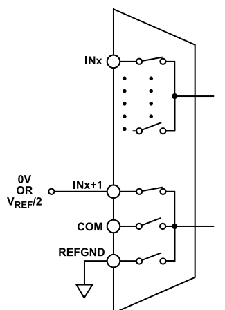
Figure 71. Even-Channel and Odd-Channel Paired
