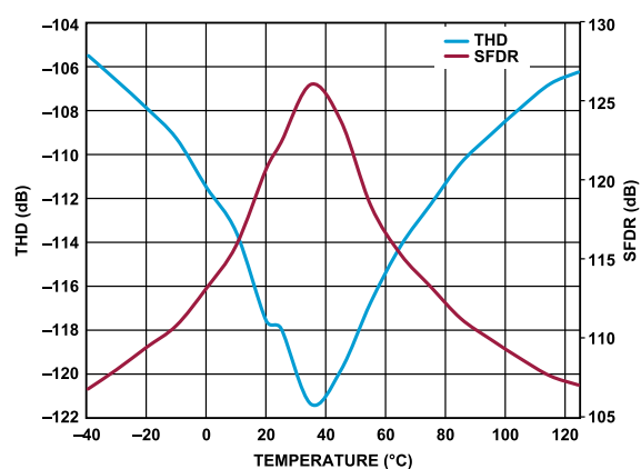
Figure 26. THD and SFDR vs. Temperature, f_{IN} = 1 kHz
