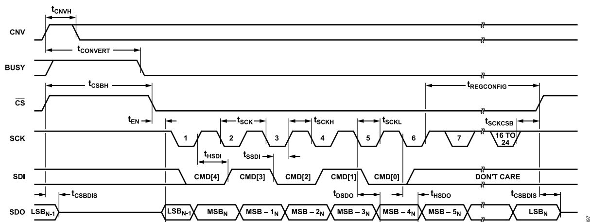
Figure 103. Conversion Mode Timing Diagram, Register Configuration Mode Command
