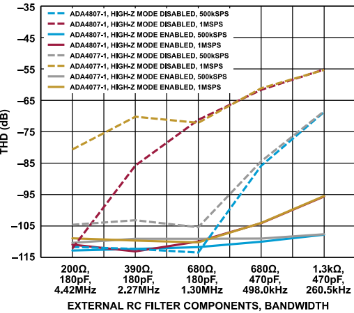
Figure 73. THD vs. External RC Filter Components, Bandwidth for Various Amplifiers ( V_{REF} = 5 V, f_{IN} = 1 kHz)
