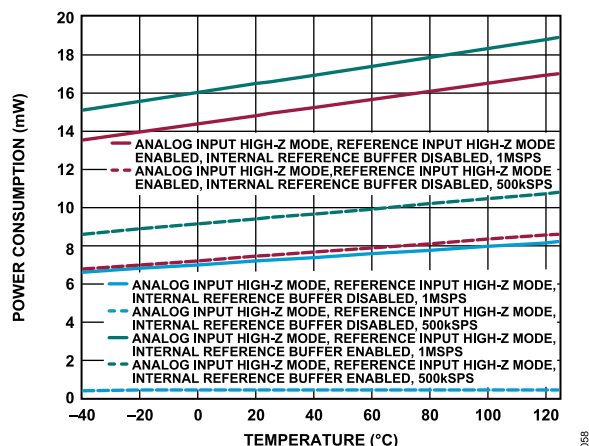
Figure 59. Power Consumption vs. Temperature, Internal LDO Disabled, f_s = 1 MSPS and 500 kSPS
