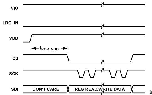
Figure 107. VDD POR Timing Diagram
