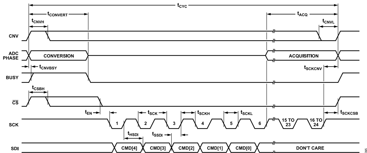
Figure 101. Conversion Mode Timing Diagram, Single-Cycle Command Mode Enabled
