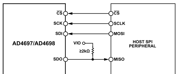
Figure 119. AD4697/AD4698 SPI Connection Diagram (Single-SDO Mode)
