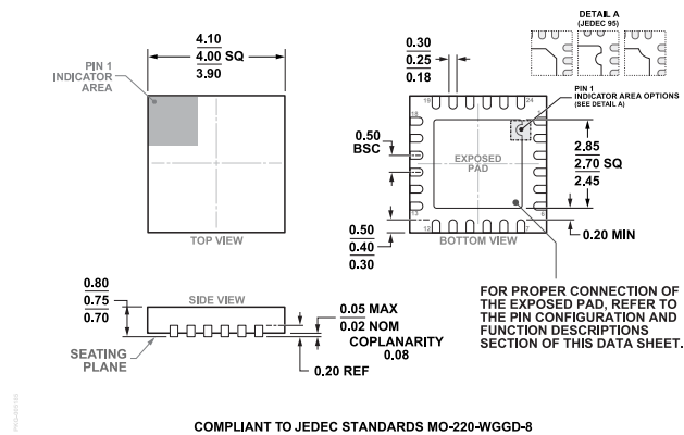
Figure 129. 24-Lead Lead Frame Chip Scale Package [LFCSP] 4 mm x 4 mm Body and 0.75 mm Package Height (CP-24-8) Dimensions shown in millimeters
