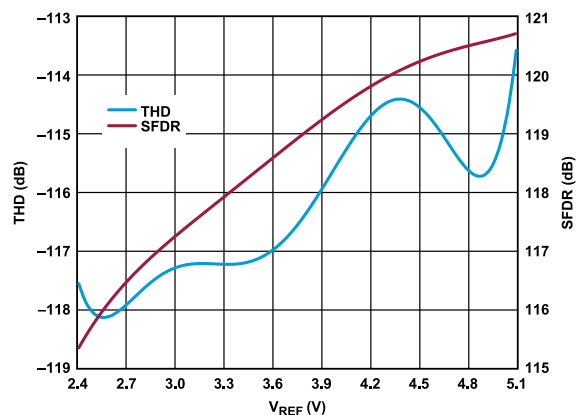
Figure 25. THD and SFDR vs. V_{REF} , f_{IN} = 1 kHz
