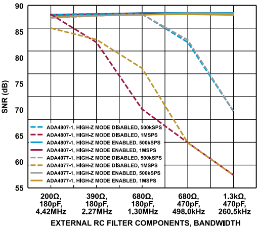
Figure 72. SNR vs. External RC Filter Components, Bandwidth for Various Amplifiers ( V_{REF} = 5 V, f_{IN} = 1 kHz)
