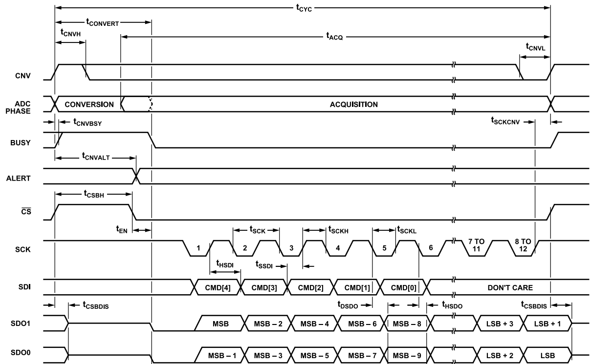
Figure 98. Conversion Mode Timing Diagram, Dual-SDO Mode, \text{SDO\_STATE} = 1
