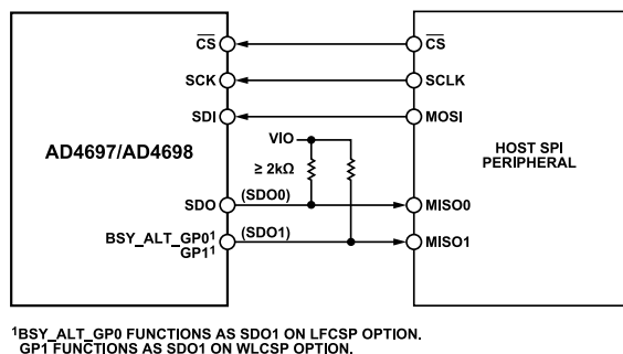
Figure 120. AD4697/AD4698 SPI Connection Diagram (Dual-SDO Mode)
