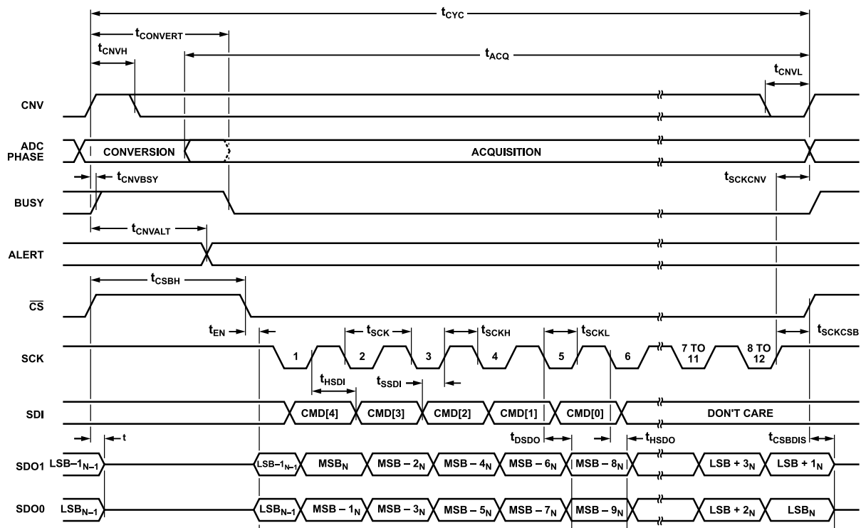
Figure 97. Conversion Mode Timing Diagram, Dual-SDO Mode, \text{SDO\_STATE} = 0
