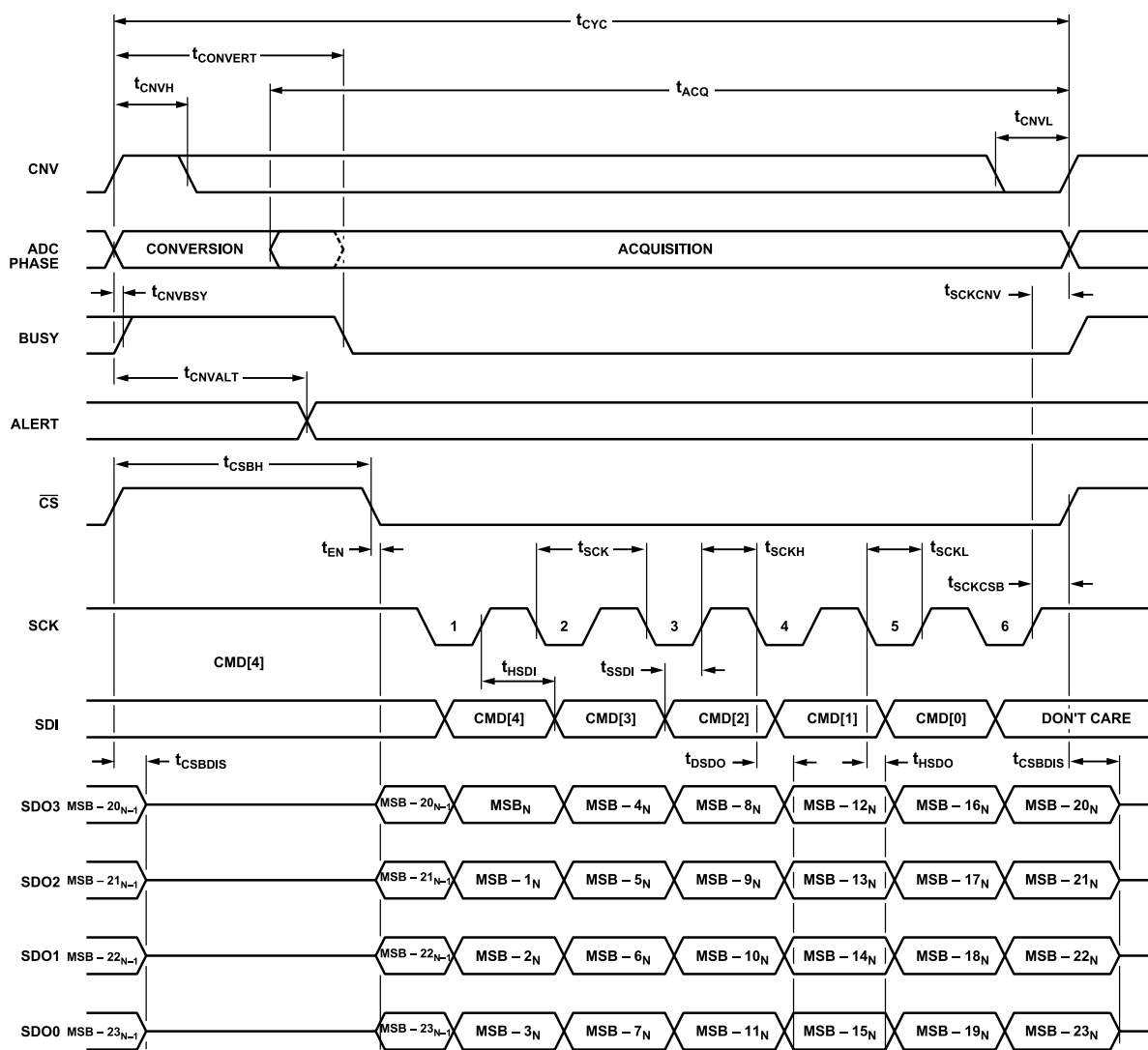
Figure 99. Conversion Mode Timing Diagram, Quad-SDO Mode, SDO\_STATE = 0
