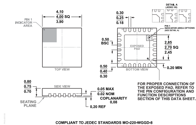
Figure 129. 24-Lead Lead Frame Chip Scale Package [LFCSP] 4 mm × 4 mm Body and 0.75 mm Package Height (CP-24-8) Dimensions shown in millimeters
