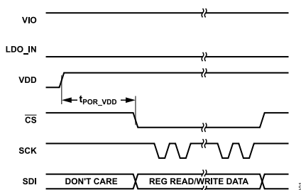
Figure 107. VDD POR Timing Diagram
