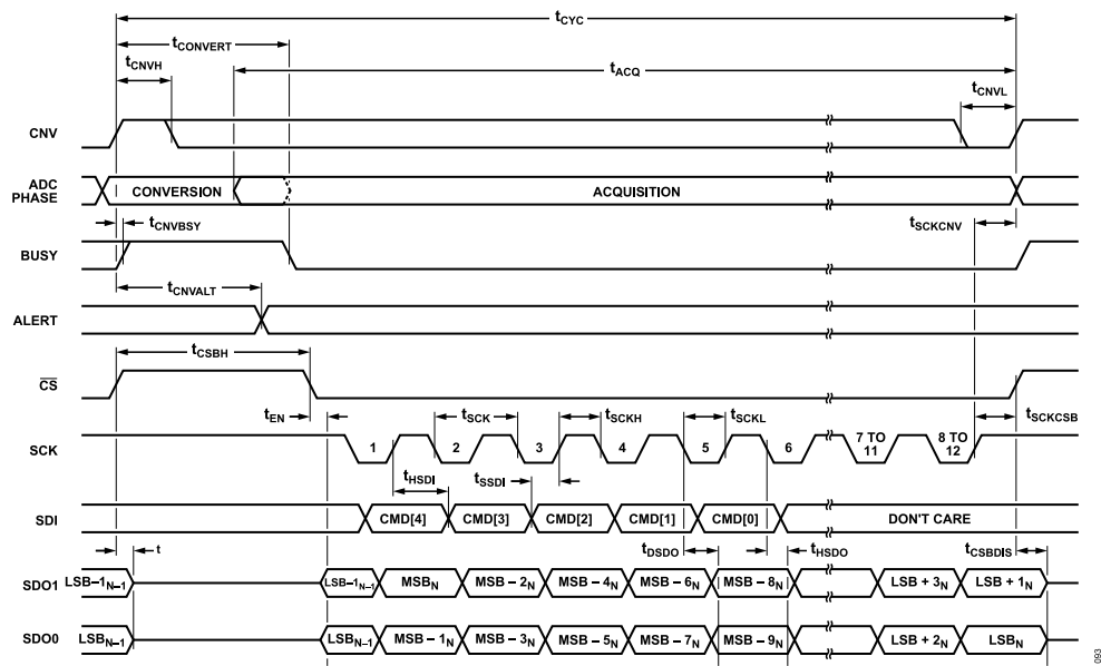
Figure 97. Conversion Mode Timing Diagram, Dual-SDO Mode, SDO_STATE = 0
