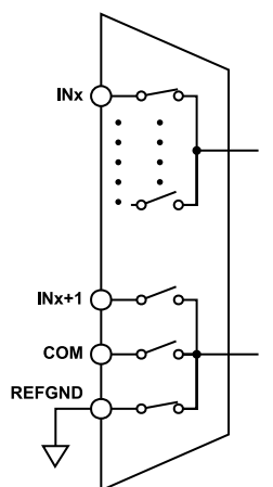
Figure 69. INx Paired with REFGND
