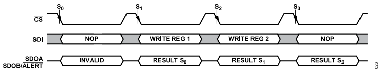
Figure 42. Register Write
