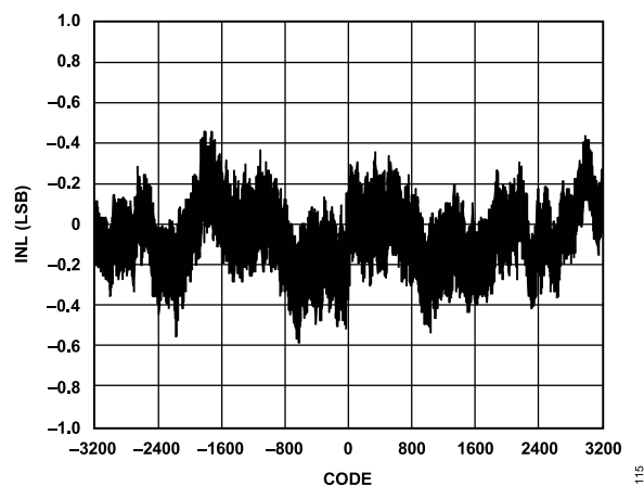
Figure 13. INL Error
