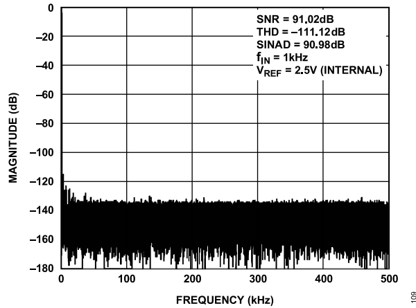
Figure 7. AD4680 Fast Fourier Transform (FFT), V_{REF} = 2.5 V Internal
