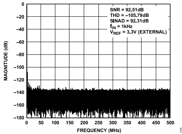
Figure 8. AD4680 FFT, V_{REF} = 3.3 V External
