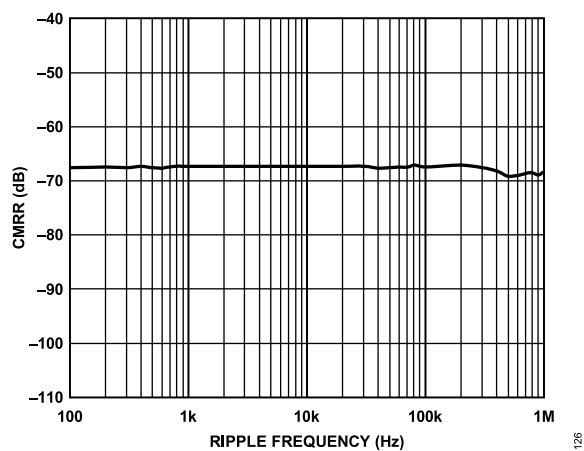
Figure 27. CMRR vs. Ripple Frequency
