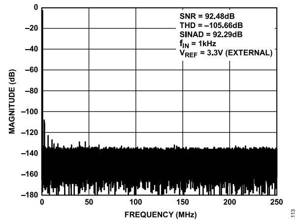
Figure 11. AD4681 FFT, V_{REF} = 3.3 V External
