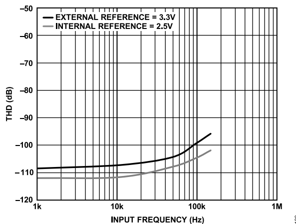
Figure 18. AD4680 THD vs. Input Frequency
