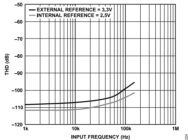
Figure 22. AD4681 THD vs. Input Frequency
