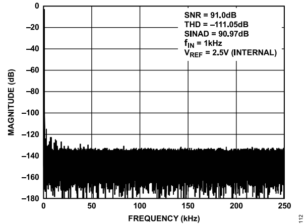
Figure 10. AD4681 FFT, V_{REF} = 2.5 V Internal
