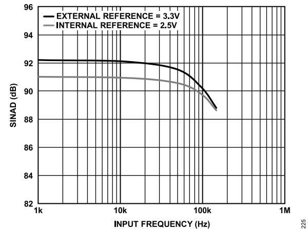
Figure 23. AD4681 SINAD vs. Input Frequency
