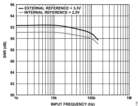
Figure 17. AD4680 SNR vs. Input Frequency
