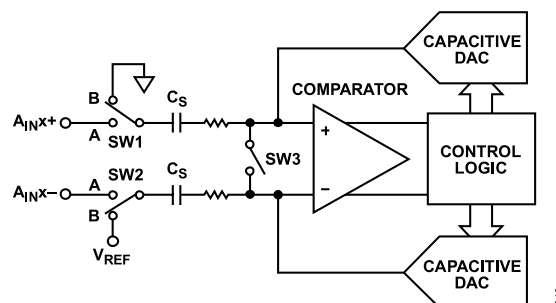
Figure 29. ADC Conversion Phase
