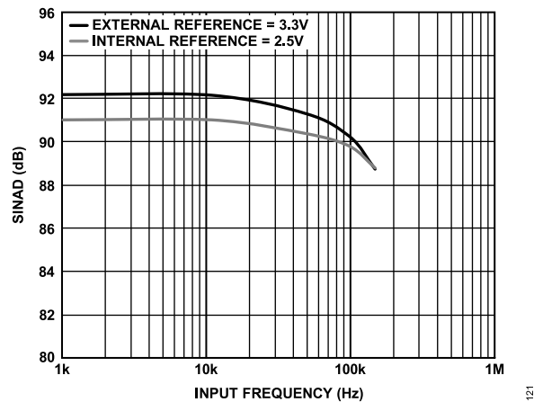
Figure 19. AD4680 SINAD vs. Input Frequency
