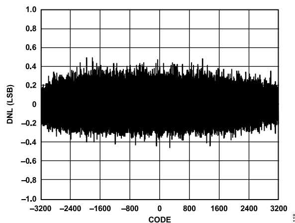
Figure 16. DNL Error
