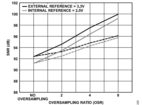
Figure 24. AD4680 SNR vs. Oversampling Ratio, Oversampling Mode
