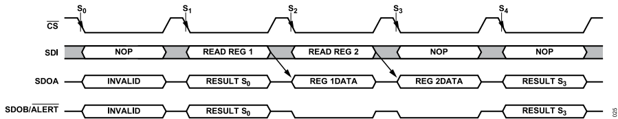
Figure 41. Register Read
