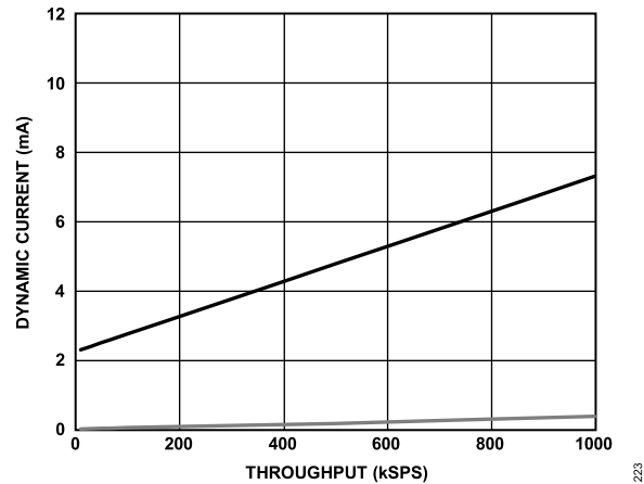
Figure 21. Dynamic Current vs. Throughput
