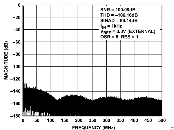
Figure 9. AD4680 FFT with Oversampling, V_{REF} = 3.3 V External
