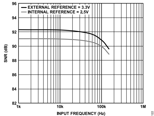
Figure 20. AD4681 SNR vs. Input Frequency
