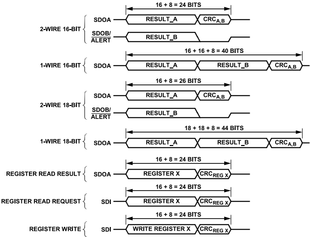
Figure 43. CRC Operation
