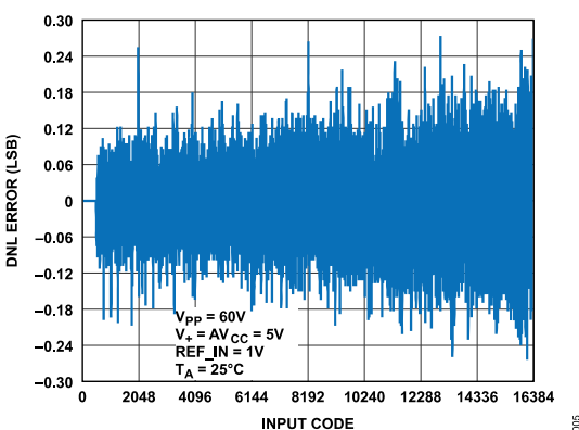
Figure 5. DNL with Full-Scale Range = 50 V
