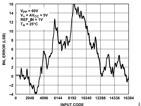
Figure 4. INL with Full-Scale Range = 50 V
