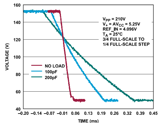
Figure 15. Settling Time Falling Edge at Various Capacitive Loads
