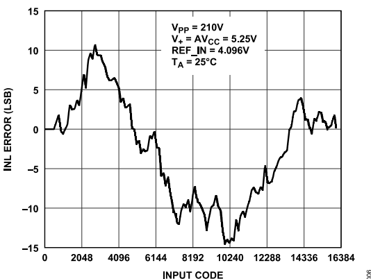
Figure 6. INL with Full-Scale Range = 200 V
