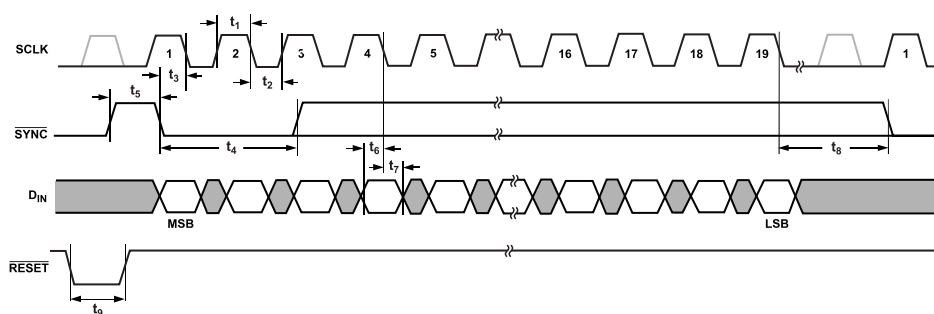
Figure 2. Serial Interface Timing Diagram
