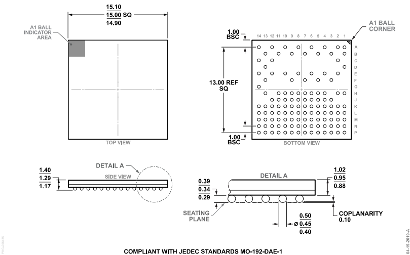
Figure 19. 124-Lead Chip Scale Package Ball Grid Array [CSP_BGA] (BC-124-4) Dimensions shown in millimeters
