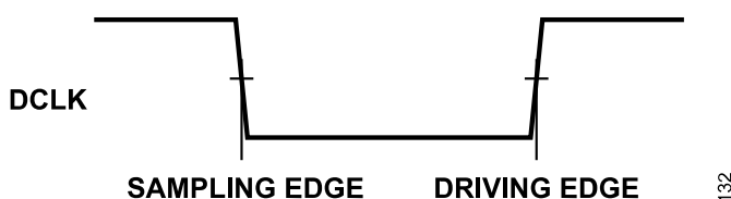
Figure 114. DCLK Edges
