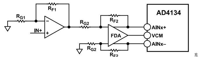
Figure 107. Op Amp and Fully Differential Amplifier
