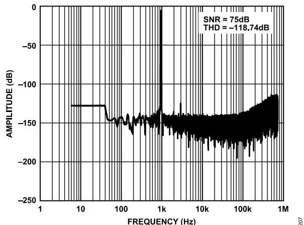
Figure 14. FFT, Low Power Mode, Sinc3 Filter, -0.5 dBFS
