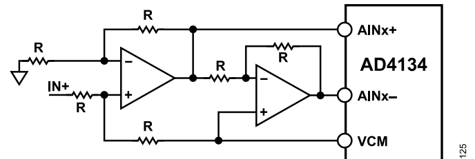
Figure 106. Dual Operation Amplifier Configuration
