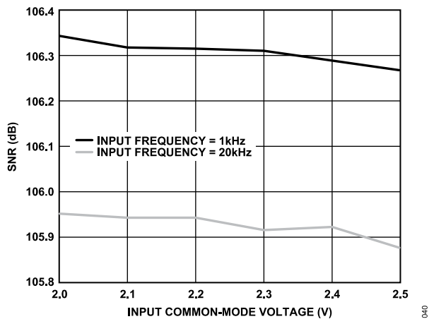
Figure 23. SNR vs. Input Common-Mode Voltage, Wideband 0.433 x ODR Filter
