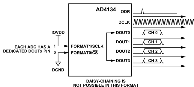
Figure 90. FORMAT1, FORMAT0 = 10, Four Data Output Pins
