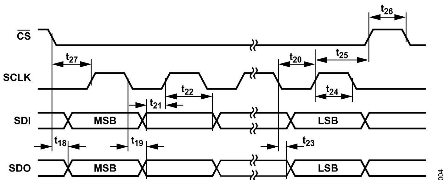
Figure 4. SPI Timing Diagram
