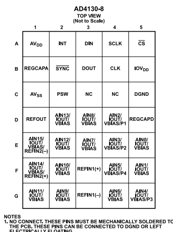
Figure 14. WLCSP Pin Configuration
