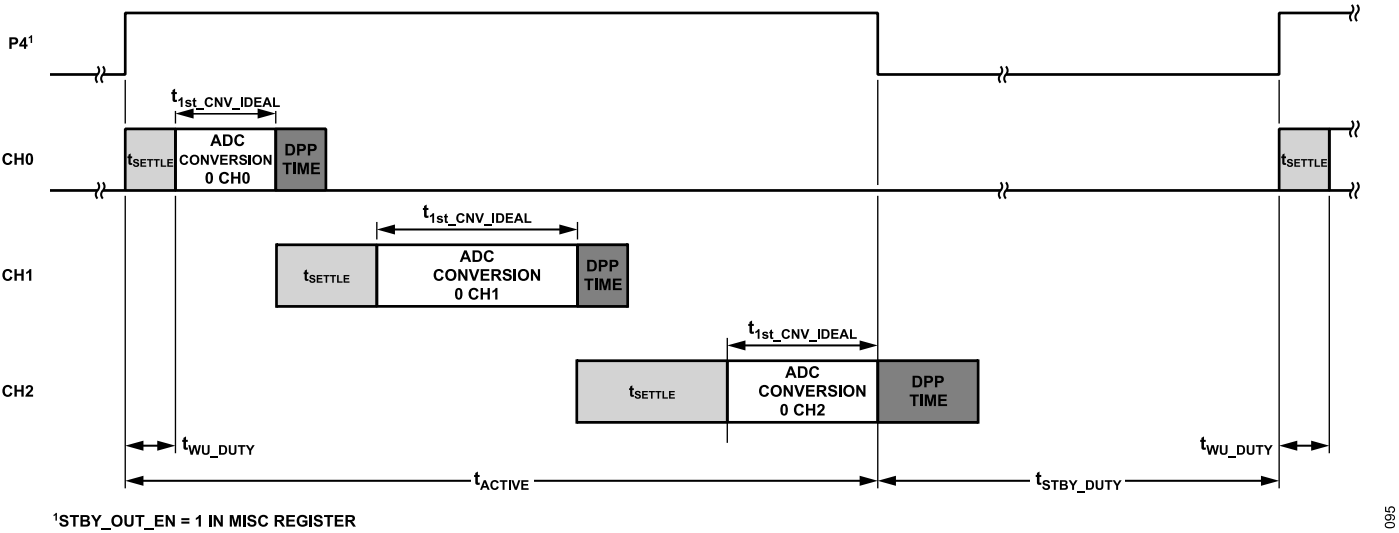
Figure 96. Example of Autonomous Duty Cycling Mode
