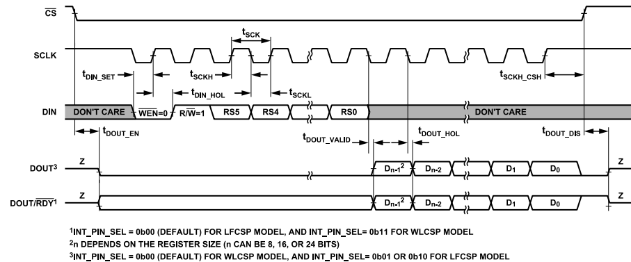
Figure 6. 3-Wire Mode Read Cycle Timing Diagram, 3-Wire Mode (CSB_EN Bit Set to 0), \overline{CS} Pin Used to Tristate the DOUT Pin
