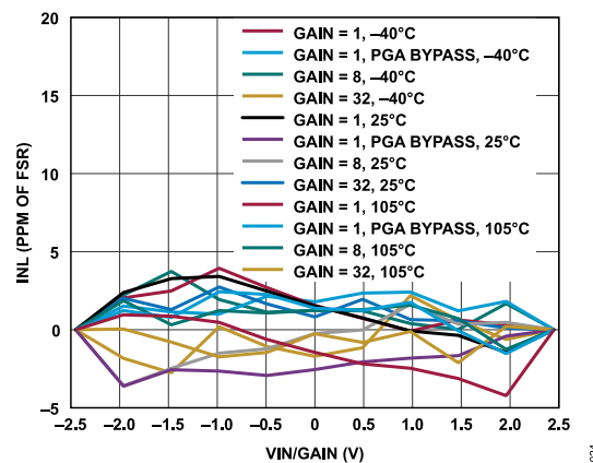
Figure 24. INL Error vs. VIN/Gain for Various Gains and Temperatures (Sinc 3 Filter, ODR = 50 SPS, Internal 2.5 V Reference)
