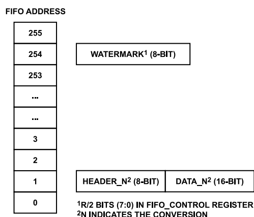
Figure 102. FIFO Structure
