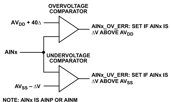
Figure 98. Analog Input Overvoltage/Undervoltage Monitors
