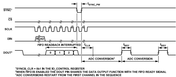
Figure 13. FIFO Clear Timing Diagram
