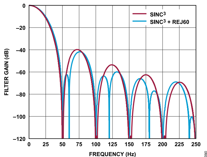
Figure 89. Sinc 3 and Sinc 3 + REJ60 Filter Response (50 SPS ODR)
