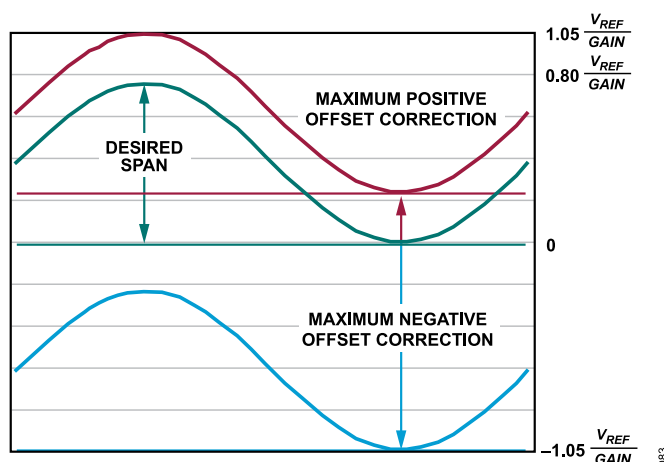
Figure 82. Example of Unipolar Span and Offset Calibration Limits
