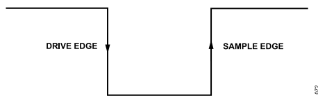
Figure 71. SPI Mode 3, SCLK Edges
