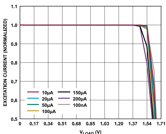
Figure 62. Output Compliance for Various IEXC Sources ( AV_{DD} = 1.71 V, V_{LOAD} is Load Voltage)
