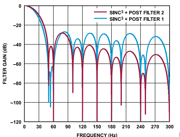
Figure 85. Post Filter 1 and Post Filter 2 Response
