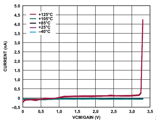
Figure 44. Differential AIN Current vs. VCM/Gain for Various Temperatures (Gain = 2 to 128, VDIFF = 0 V)
