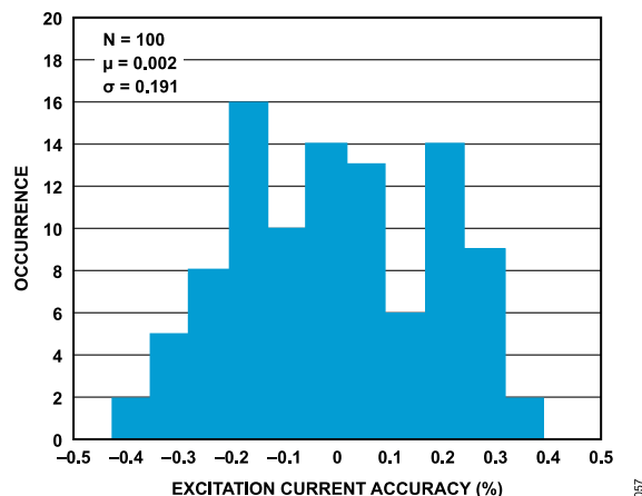
Figure 57. Excitation Current Initial Accuracy Histogram (100 µA)
