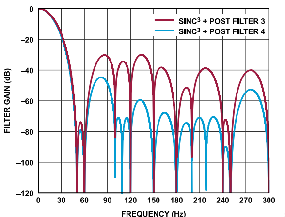
Figure 86. Post Filter 3 and Post Filter 4 Response
