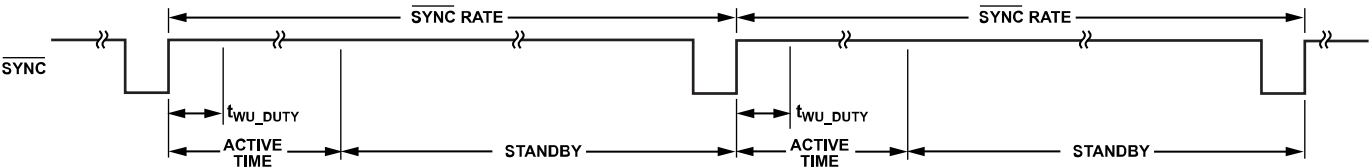
Figure 78. Example of Single Sequence + STBY by \overline{SYNC} Mode Diagram
