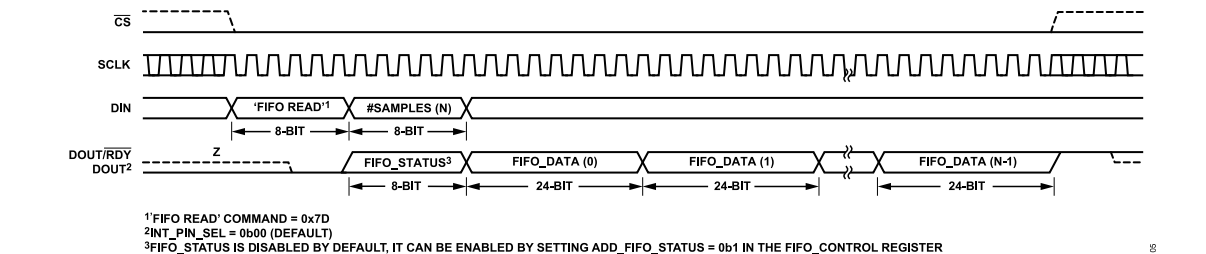
Figure 104. FIFO Readback (FIFO_STATUS Append On and FIFO_HEADER Append Off)
