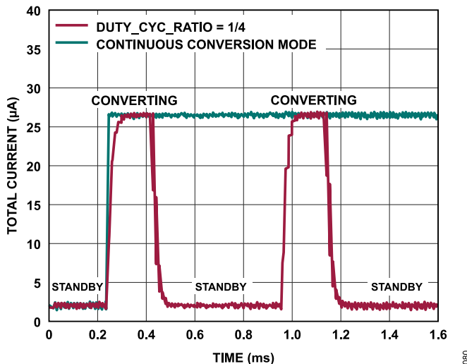
Figure 79. Example of Duty Cycling Mode vs. Continuous Conversion Mode Current Consumption
