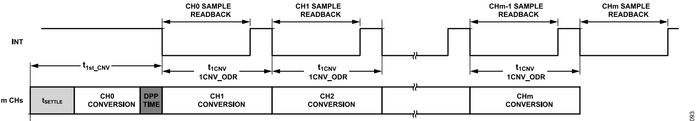
Figure 92. Example of Standard Sequencing Through Multiple Channels with Same Configuration and No Repeat Conversion
