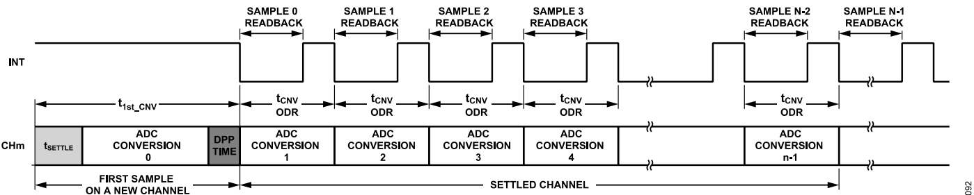
Figure 91. Example of Repeat Conversion on the Same Channel
