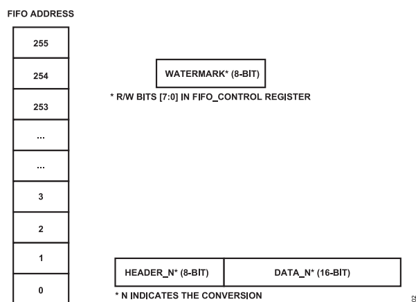
Figure 101. FIFO Structure
