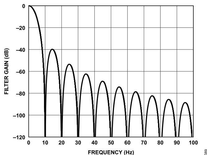
Figure 88. Simultaneous 50 Hz and 60 Hz Rejection for Sinc 3 with ODR = 10 SPS
