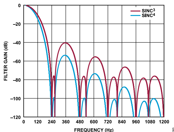
Figure 84. Sinc 3 and Sinc 4 Filter Response (FS = 0d10)
