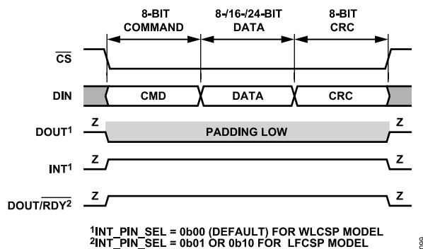
Figure 98. SPI Write Transaction with CRC
