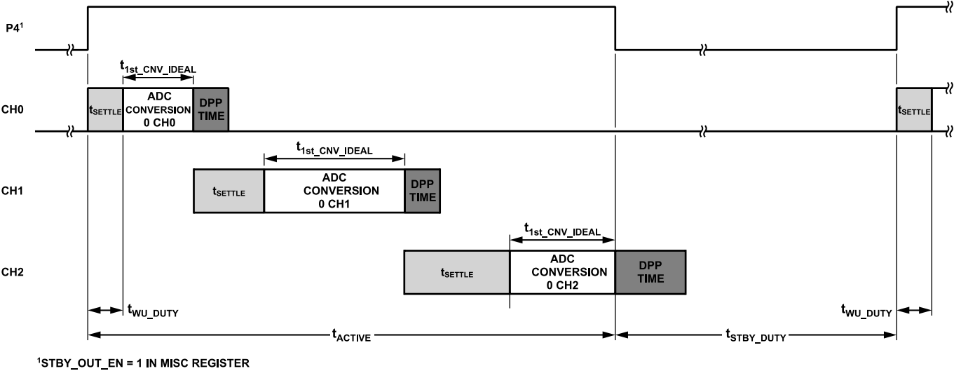
Figure 94. Example of Autonomous Duty Cycling Mode
