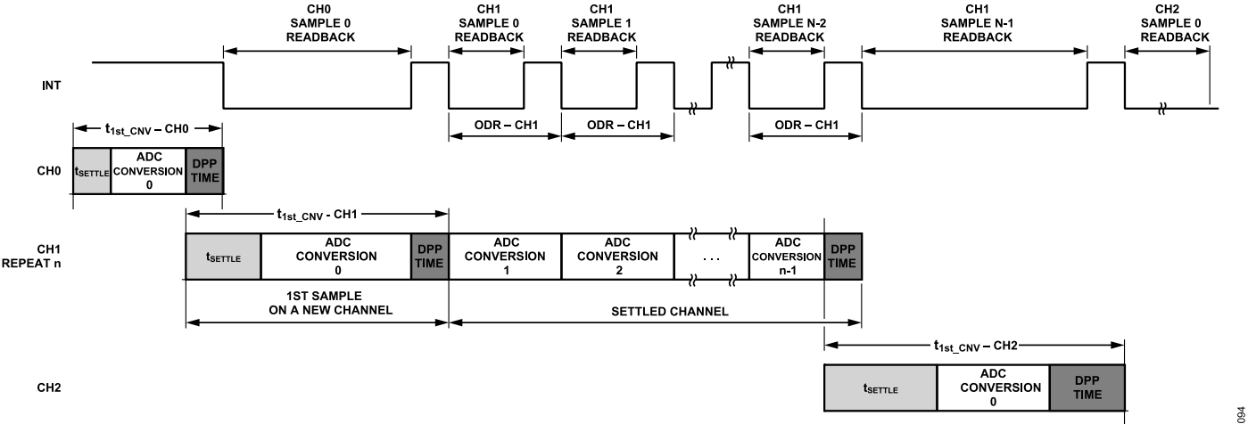
Figure 93. Example of Smart Sequencing
