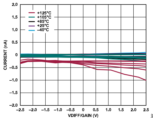
Figure 42. Absolute AINM Current vs. VDIFF/Gain for Various Temperatures (Gain = 2 to 128, VCM = AV_{DD}/2 )
