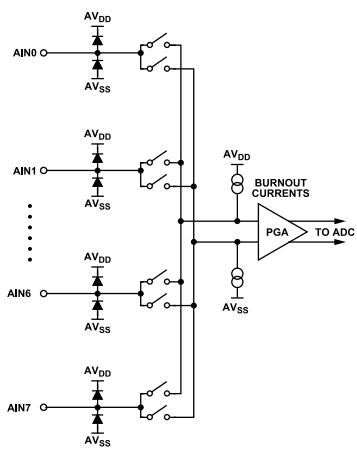
Figure 69. Analog Input Multiplexer Circuit
