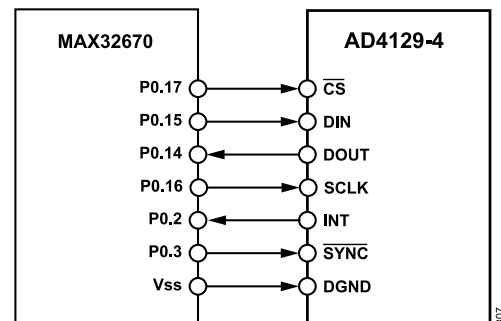
Figure 106. Example of MAX32670 \mu C SPI Connection to AD4129-4
