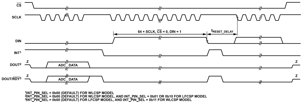
Figure 74. Software Reset Timing Diagram
