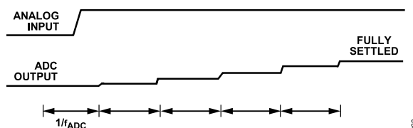
Figure 87. Effect of an Asynchronous Step Change in the Analog Input on the ADC Output
