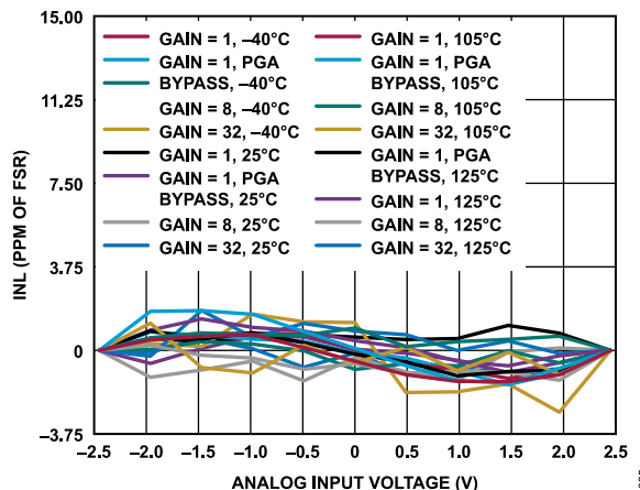
Figure 25. INL Error vs. Differential Input Amplitude for Various Gains and Temperatures (Sinc 3 Filter, ODR = 50 SPS, External 2.5 V Reference)
