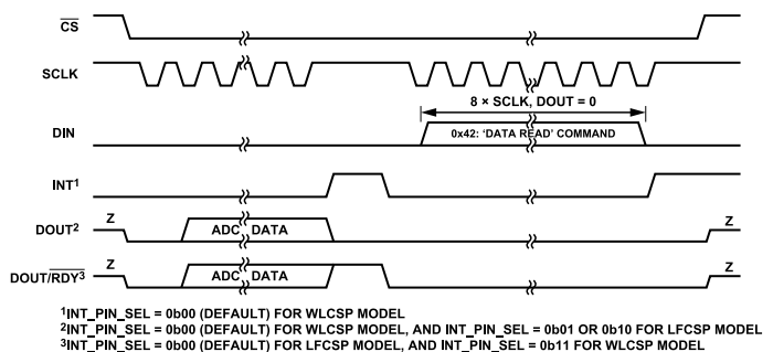
Figure 81. Exit Continuous Read Mode Diagram (CRC Disabled)
