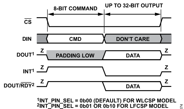
Figure 73. Reading from a Register (8-Bit Command with Register Address Followed by Data)
