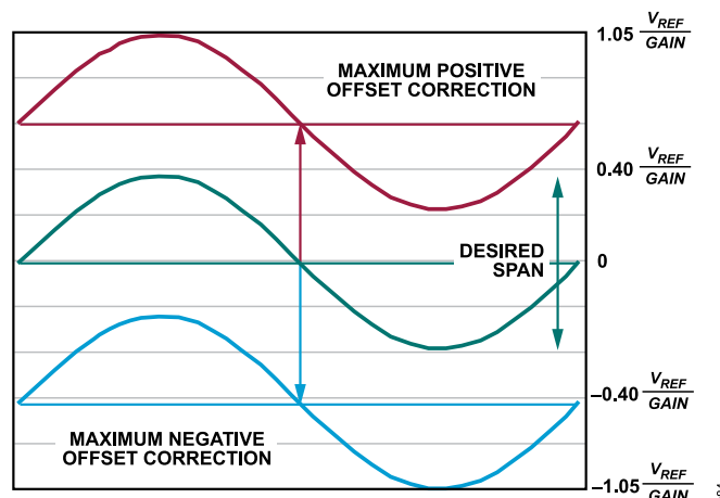
Figure 83. Example of Bipolar Span and Offset Calibration Limits
