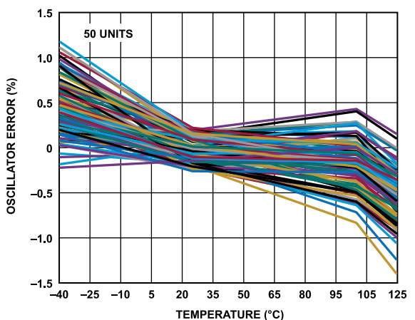
Figure 26. Internal Oscillator Error vs. Temperature
