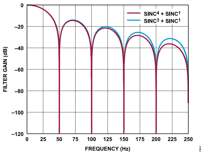
Figure 90. Sinc 3 + Sinc 1 and Sinc 4 + Sinc 1 Filter Response (FS = 6)
