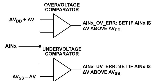
Figure 97. Analog Input Overvoltage/Undervoltage Monitors
