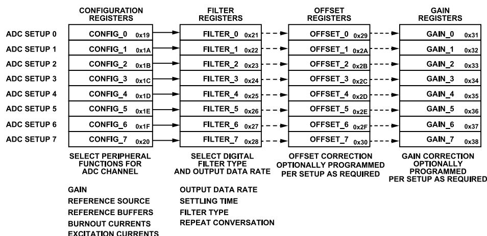
Figure 75. ADC Setup Register Grouping
