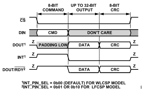
Figure 99. SPI Read Transaction with CRC
