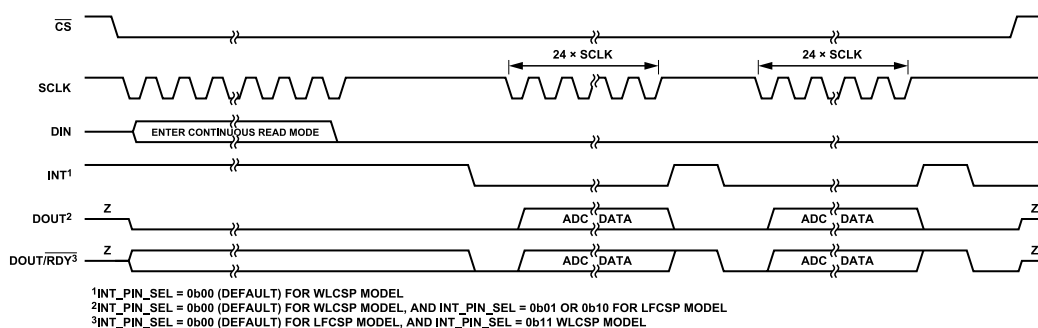
Figure 80. Enter Continuous Read Mode Diagram ( DATA_STATUS = 0)
