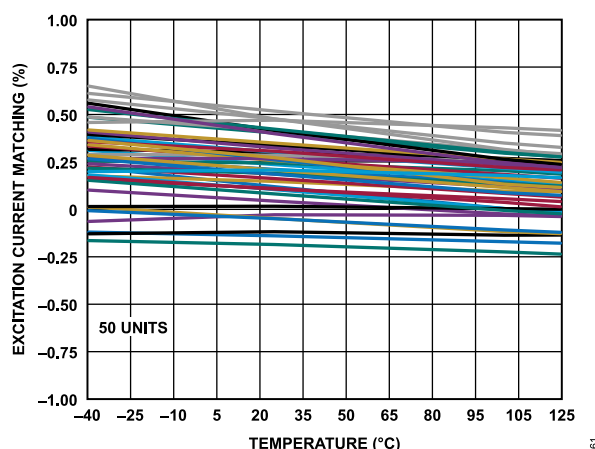
Figure 61. Excitation Current Matching vs. Temperature (100 µA)
