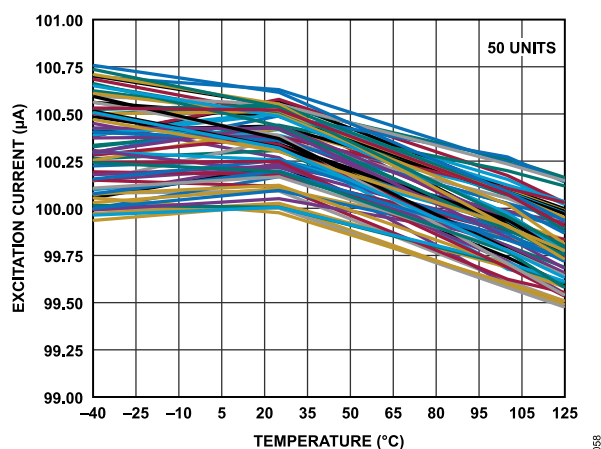
Figure 58. Excitation Current vs. Temperature (100 µA)
