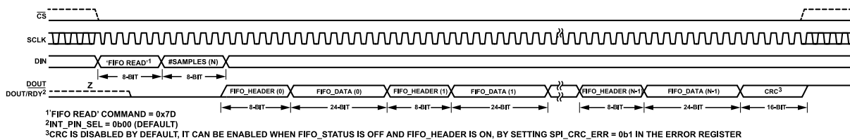
Figure 105. FIFO Readback (FIFO_STATUS Append Off and FIFO_HEADER Append On, CRC On)
