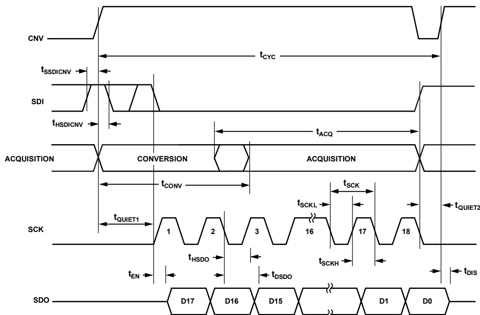
Figure 58. \overline{CS} Mode, 4-Wire Turbo Mode Timing Diagram (Status Bits Not Shown)
