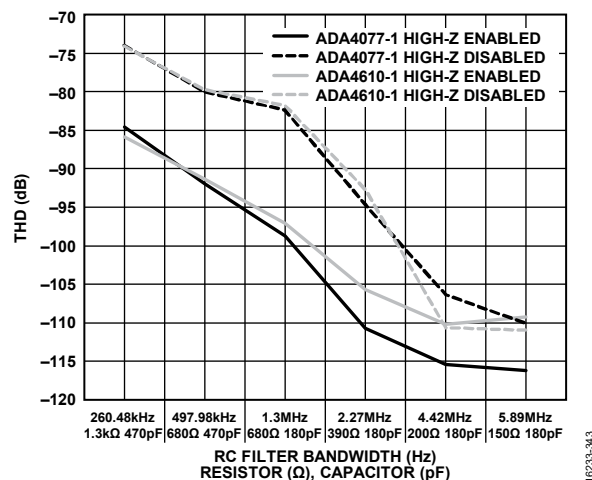
Figure 46. THD vs. RC Bandwidths for Various Precision ADC Drivers, f_{IN} = 1 kHz (Turbo Mode On, High-Z Enabled/Disabled), V_{DD} = 1.8 V, V_{IO} = 3.3 V, V_{REF} = 5 V, T_A = 25°C
