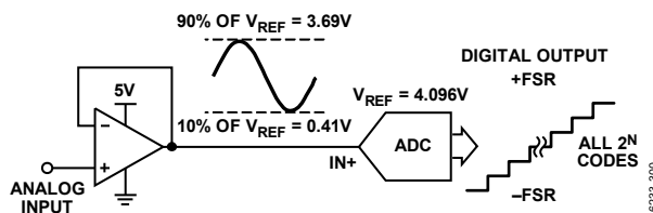
Figure 44. Span Compression
