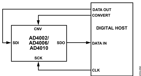
Figure 51. \overline{CS} Mode, 3-Wire Turbo Mode Connection Diagram
