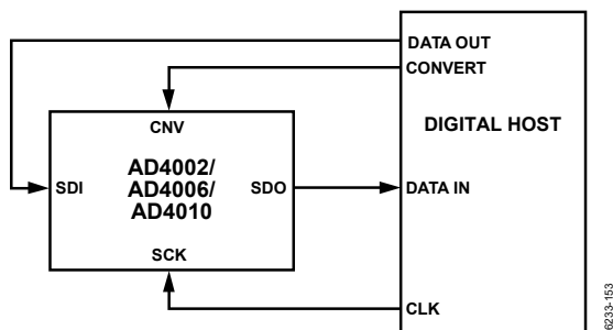
Figure 57. \overline{CS} Mode, 4-Wire Turbo Mode Connection Diagram
