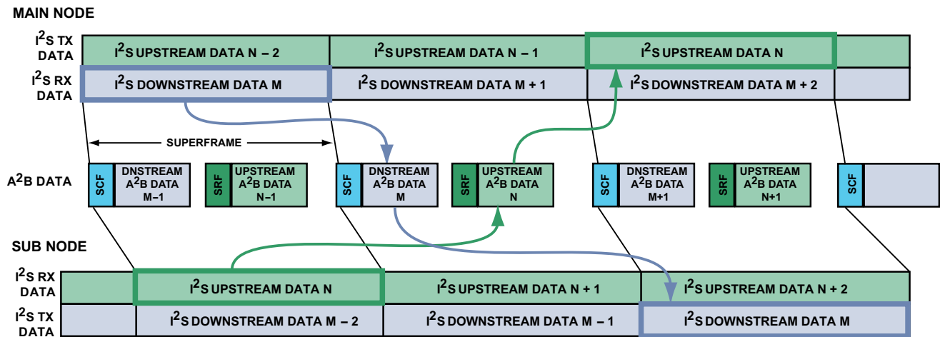
Figure 4. A²B Bus Synchronous Data Exchange
