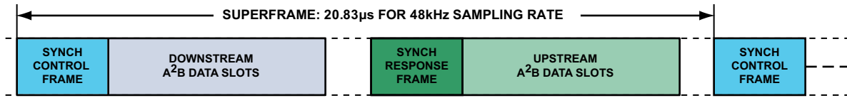
Figure 3. A²B Superframe
