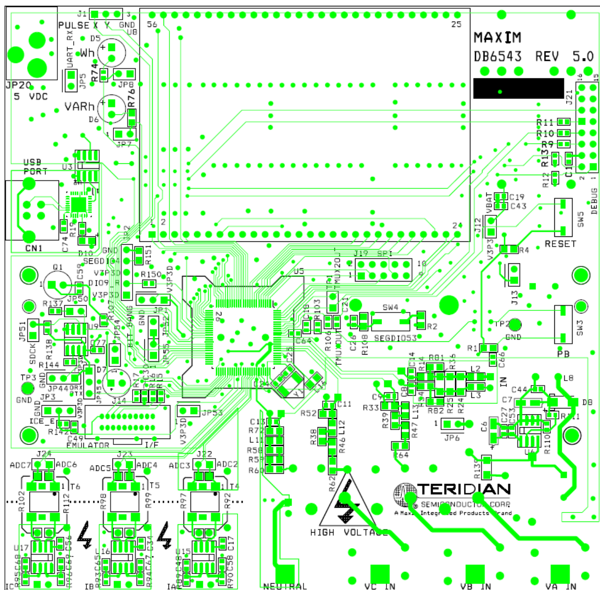
Figure 4-14: Teridian 71M6543 REV 5.0 Demo Board: Top View
