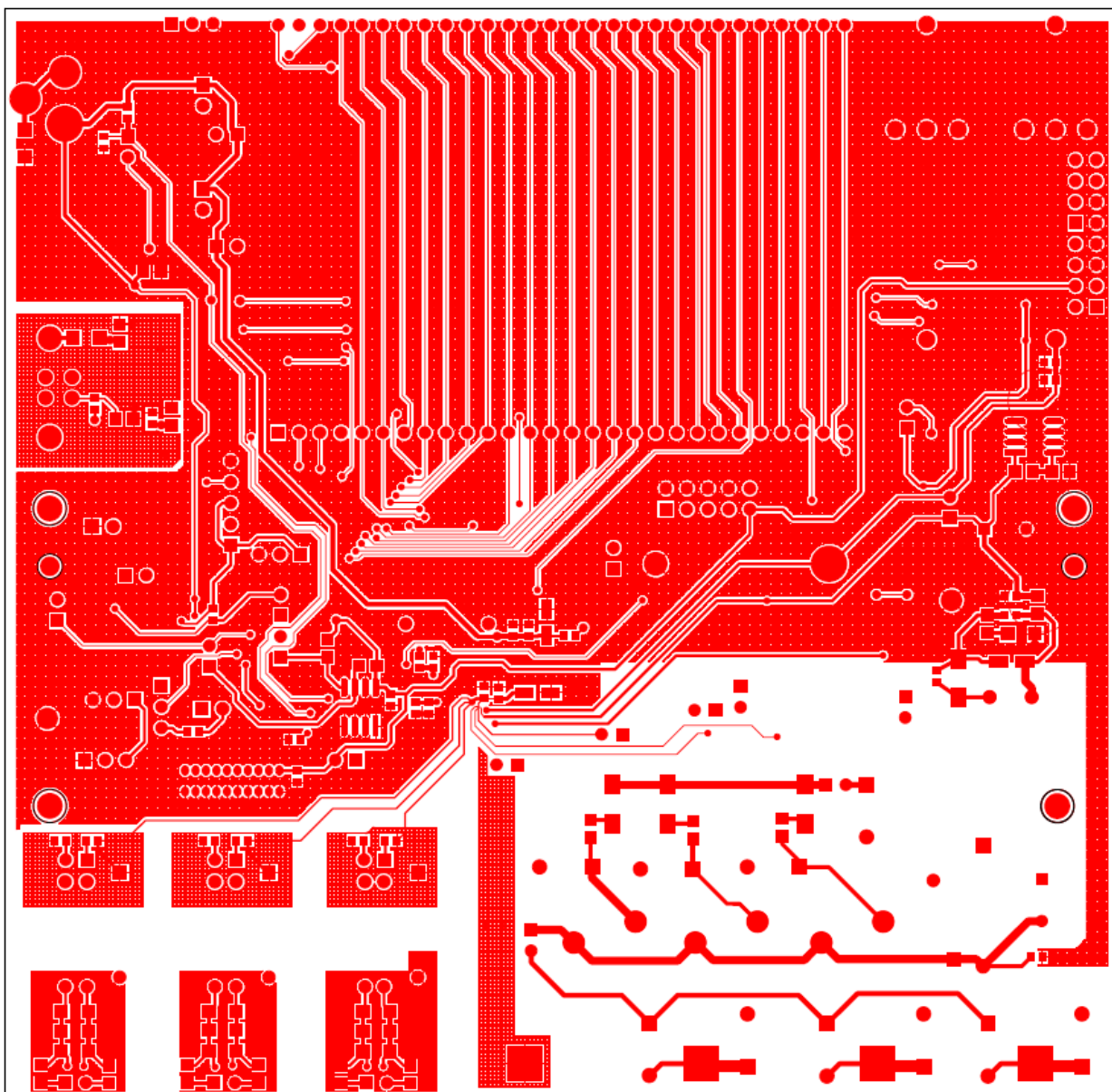
Figure 4-17: Teridian 71M6543 REV 5.0 Demo Board: Bottom Copper
