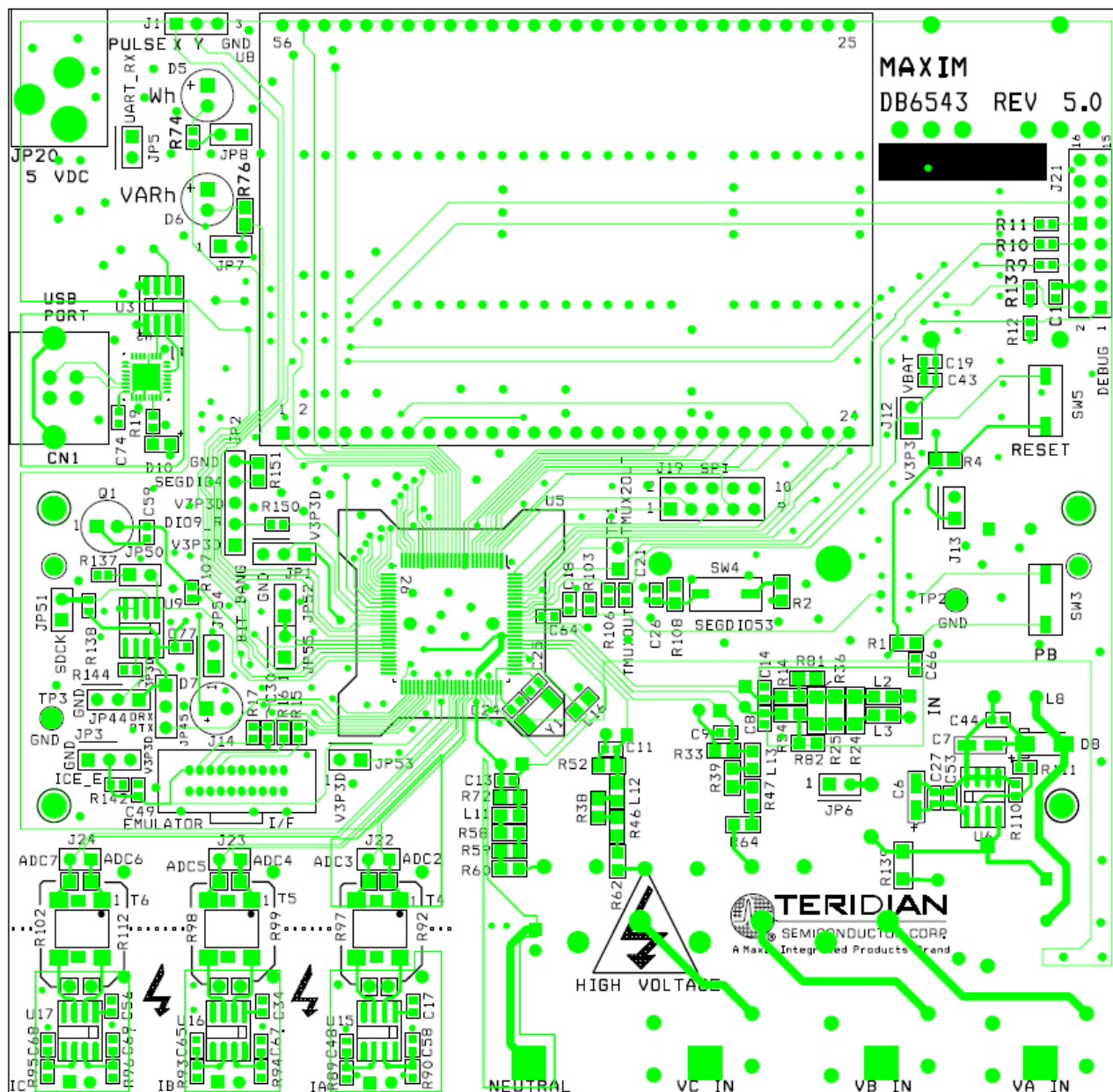
Figure 3-2: 71M6543 REV 5.0 Demo Board – Top View
