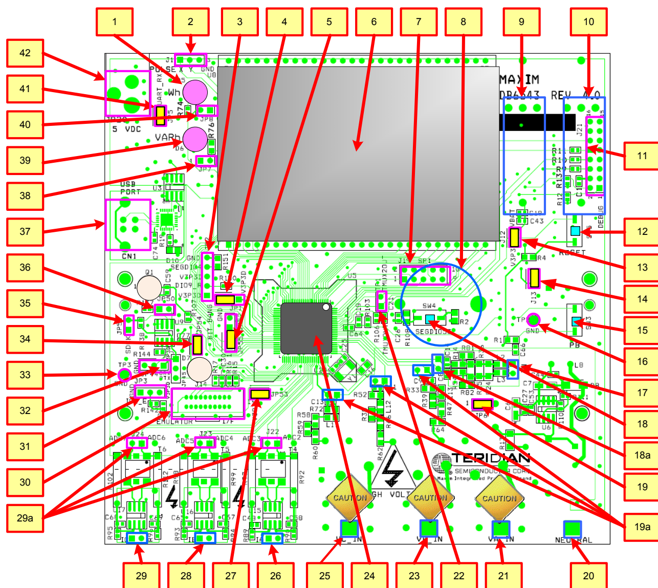
Figure 3-1: 71M6543 REV 4.0 Demo Board - Board Description
