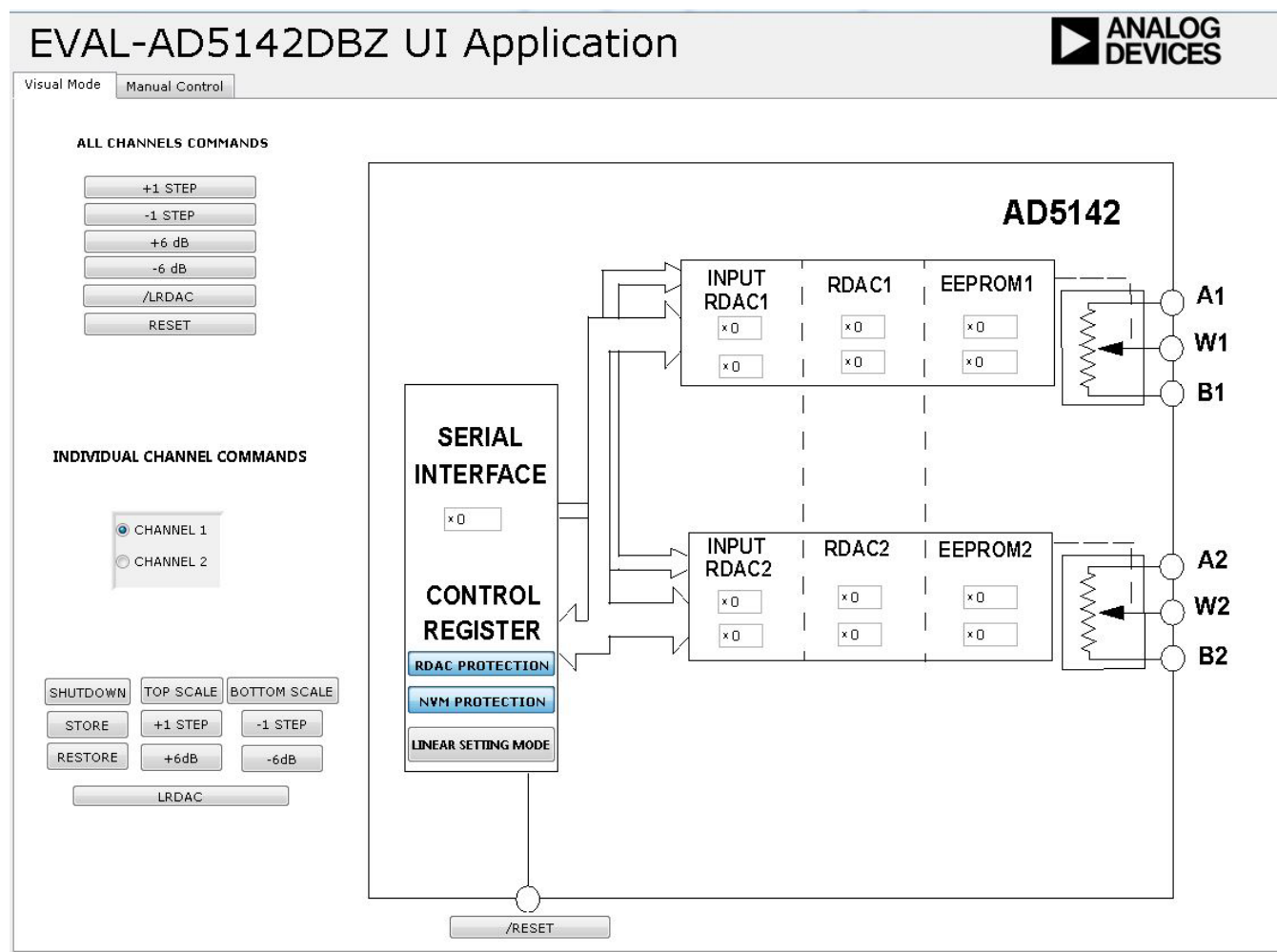
Figure 9. EVAL-AD5142DBZ Software Main Window
