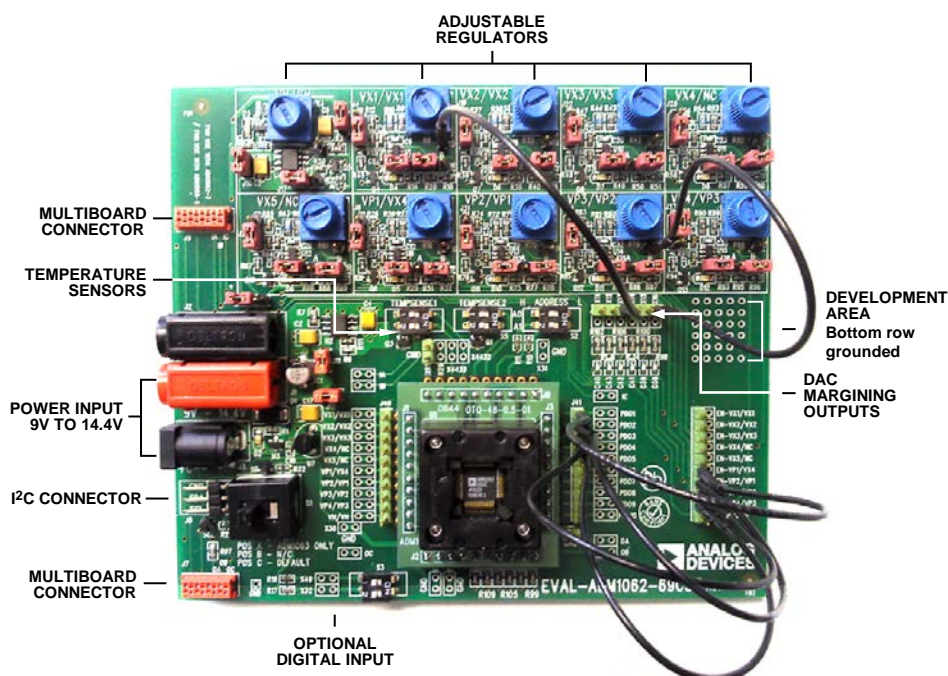
Figure 1. Evaluation Board Wiring with Point-To-Point Patch Cables
