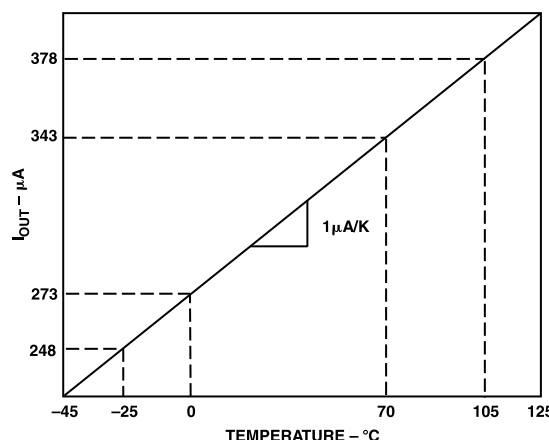
Figure 1. Transfer Characteristic
