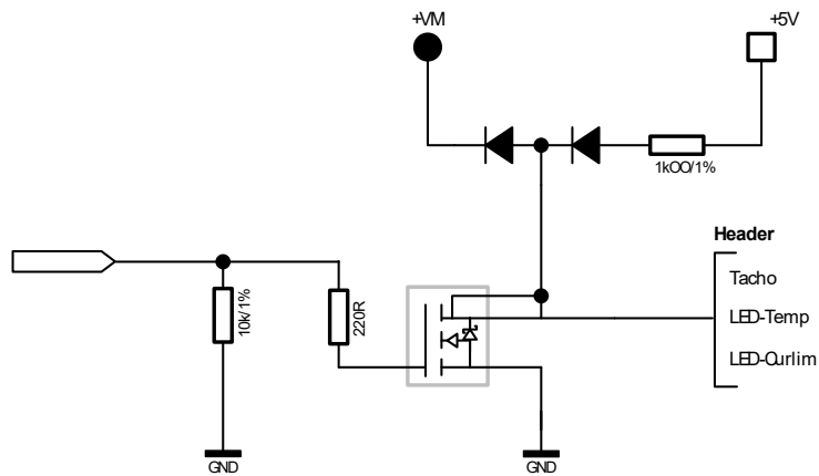
Figure 5.4: Internal circuit of the outputs
