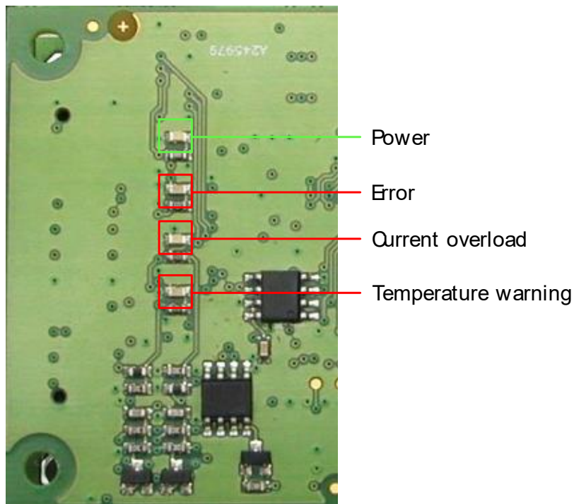
Figure 6.1: On-board LEDs
