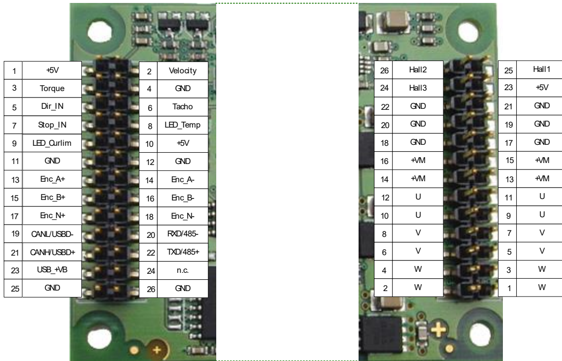
Figure 5.1: Connectors
