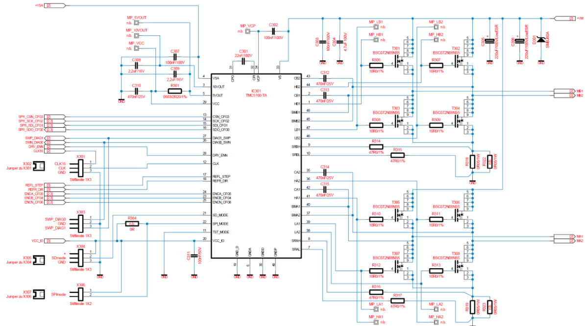
Schematic (TMC5160+MOSFETs shown)
