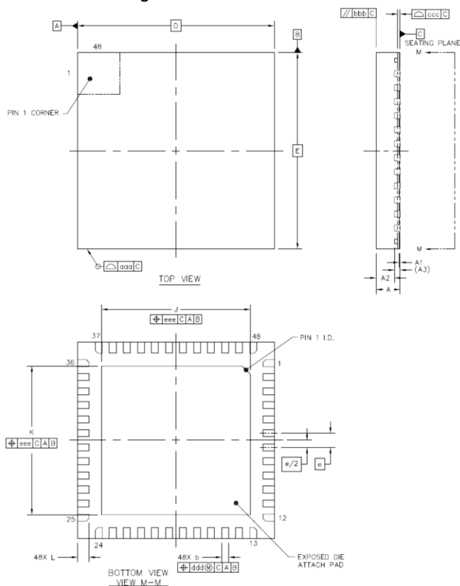
Figure 19.1 Dimensional drawings
