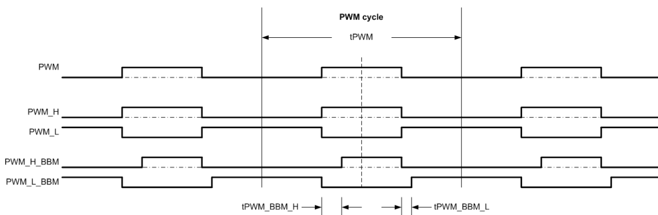
Figure 38: BBM Timing
