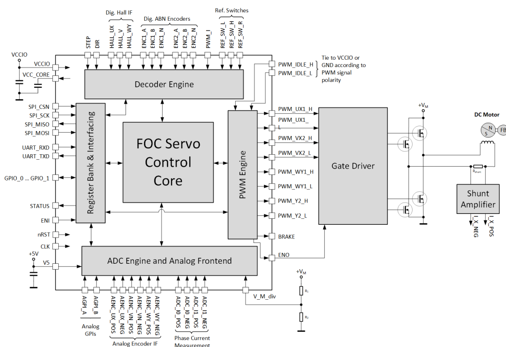
Figure 41: TMC4671 Pinout with DC Motor or Voice Coil
