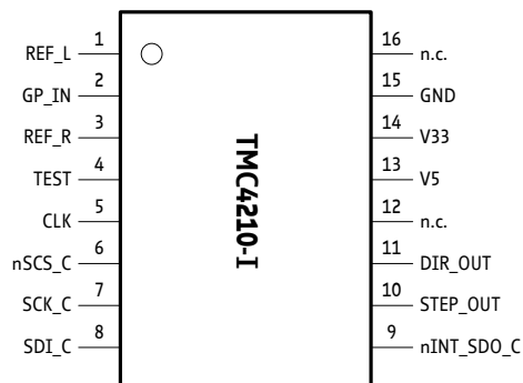
SSOP16 (150 MILS)
