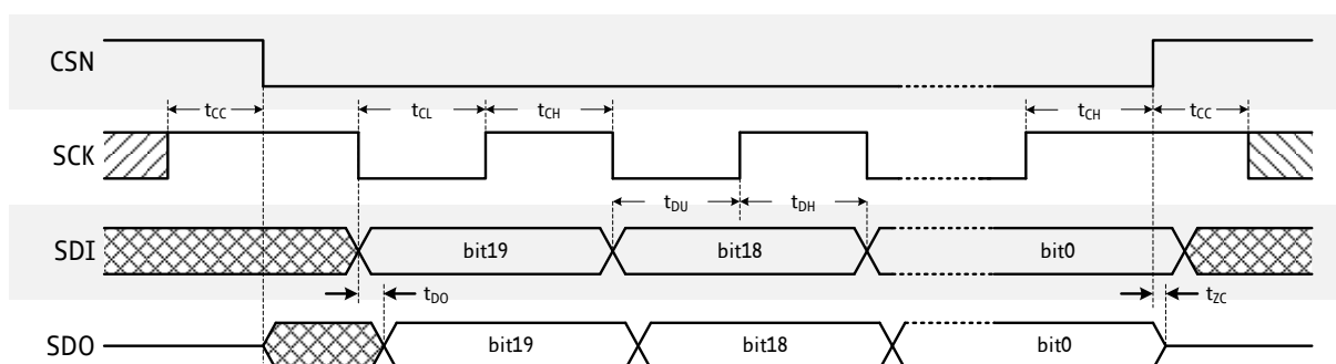
Figure 7.1 SPI Timing
