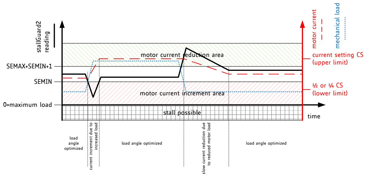
Figure 6.2 CoolStep adapts motor current to the load.
