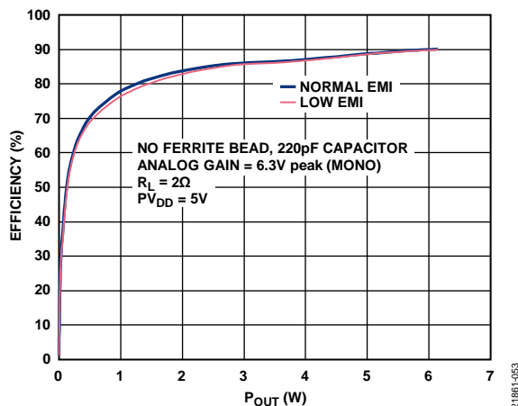
Figure 55. Efficiency vs. P_{OUT} , No Ferrite Bead, Analog Gain = 6.3 V peak, R_L = 2\ \Omega , PV_{DD} = 5\text{ V}
