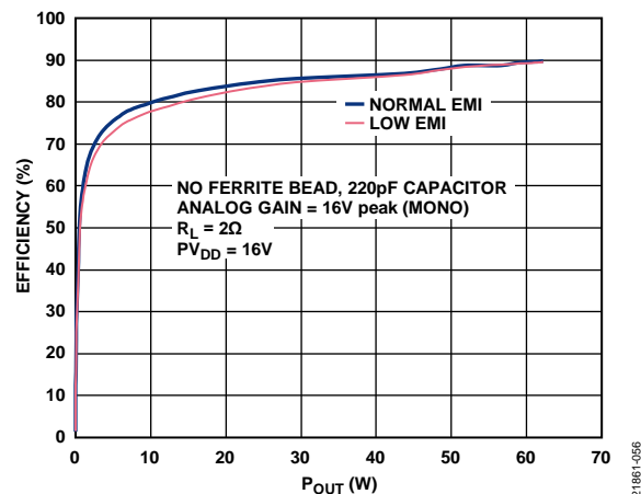
Figure 58. Efficiency vs. P_{OUT} , No Ferrite Bead, Analog Gain = 16 V peak, R_L = 2\ \Omega , PV_{DD} = 16\text{ V}
