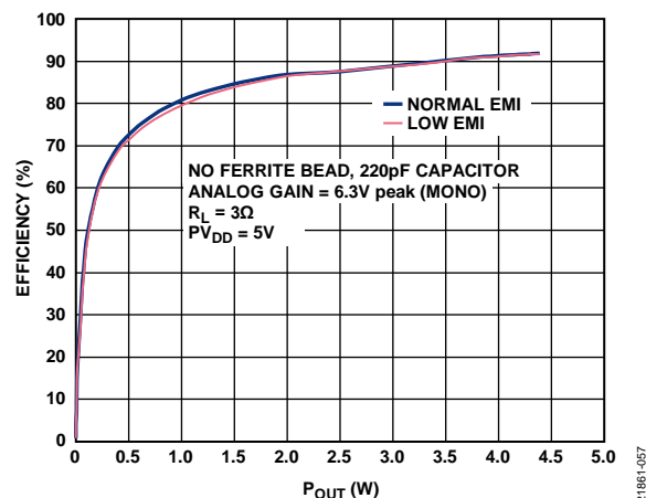
Figure 59. Efficiency vs. P_{OUT} , No Ferrite Bead, Analog Gain = 6.3 V peak, R_L = 3\ \Omega , PV_{DD} = 5\text{ V}
