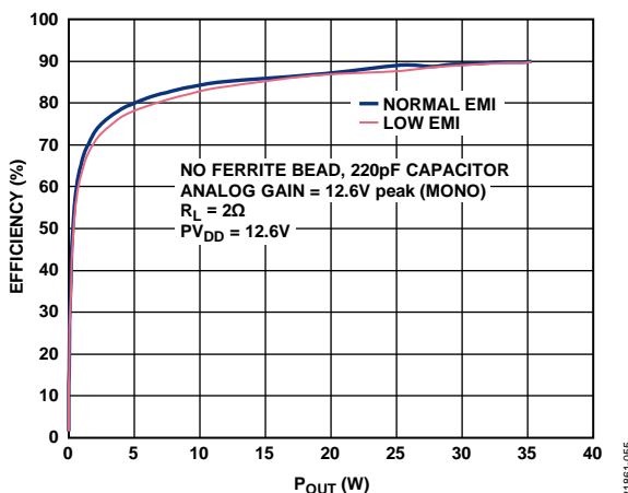
Figure 57. Efficiency vs. P_{OUT} , No Ferrite Bead, Analog Gain = 12.6 V peak, R_L = 2\ \Omega , PV_{DD} = 12.6\text{ V}
