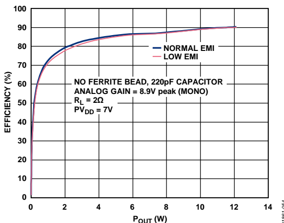
Figure 56. Efficiency vs. P_{OUT} , No Ferrite Bead, Analog Gain = 8.9 V peak, R_L = 2\ \Omega , PV_{DD} = 7\text{ V}
