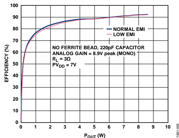
Figure 60. Efficiency vs. P_{OUT} , No Ferrite Bead, Analog Gain = 8.9 V peak, R_L = 3\ \Omega , PV_{DD} = 7\text{ V}
