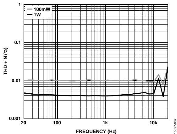
Figure 15. THD + N vs. Frequency into R_L = 4\ \Omega , PV_{DD} = 4.5\ V
