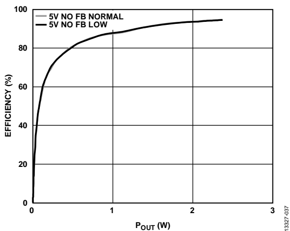
Figure 45. Efficiency vs. P_{OUT} , R_L = 8\ \Omega , No FB and 220 pF Capacitor, P_{VDD} = 5\ \text{V} , Analog Gain = 8.4
