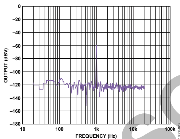
Figure 28. Output Spectrum vs. Frequency, PVDD = 3.0V , R_L = 32\Omega
