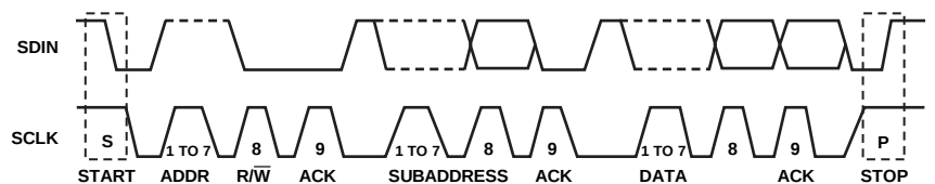
Figure 24. 2-Wire I 2 C Generalized Clocking Diagram
