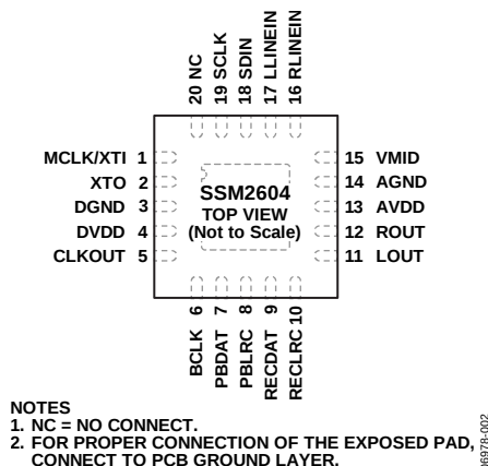
Figure 6. Pin Configuration
