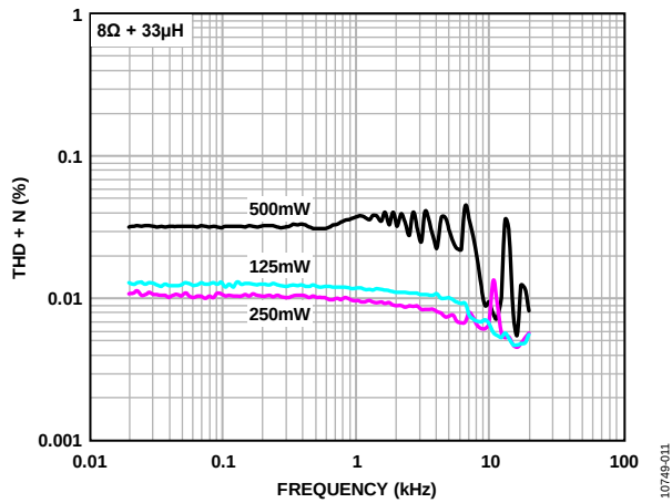
Figure 11. THD + N vs. Frequency into 8 Ω, SPVKDD = 3.6 V
