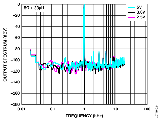
Figure 23. Output Spectrum vs. Frequency (FFT with 100 mW Output Power into 8\Omega Load)
