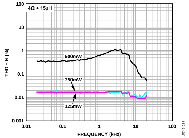
Figure 14. THD + N vs. Frequency into 4 Ω, SPVKDD = 2.5 V
