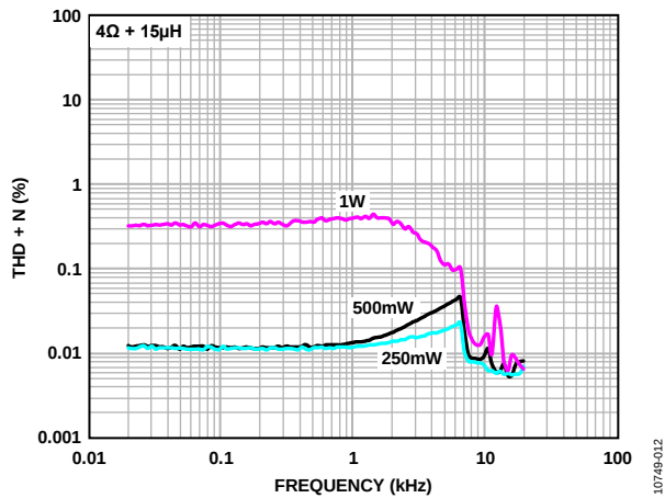
Figure 12. THD + N vs. Frequency into 4 Ω, SPVKDD = 3.6 V
