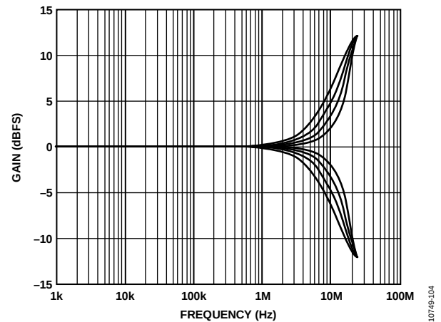
Figure 35. Treble Band Frequency Response Across Bandwidth Settings
