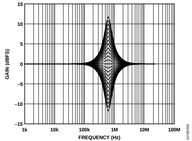
Figure 33. Peak Filter Frequency Response Across Gain Settings
