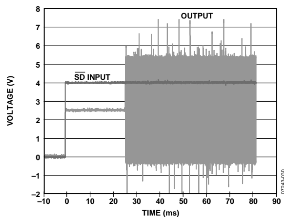
Figure 30. Turn-On Response
