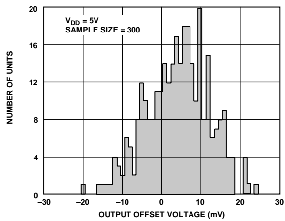
Figure 38. Output Offset Voltage Distribution
