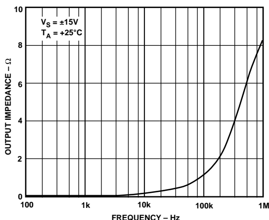
Figure 12. Closed-Loop Output Impedance vs. Frequency
