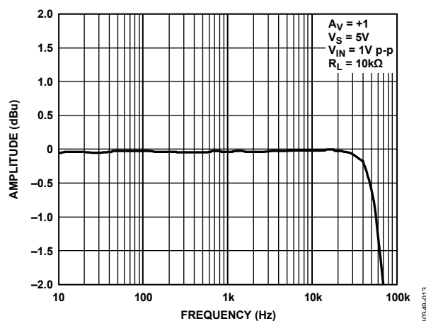
Figure 13. Frequency Response
