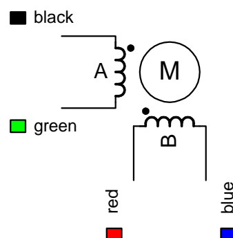
Figure 3.1: Lead wire configuration
