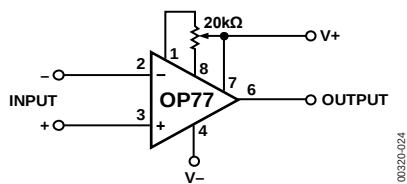
Figure 23. Optional Offset Nulling Circuit
