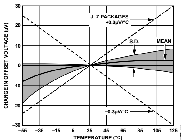
Figure 6. Untrimmed Offset Voltage vs. Temperature
