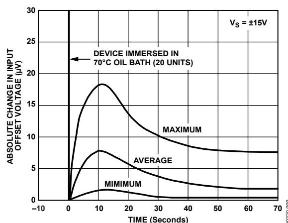
Figure 8. Offset Voltage Change Due to Thermal Shock
