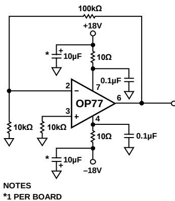
Figure 24. Burn-In Circuit
