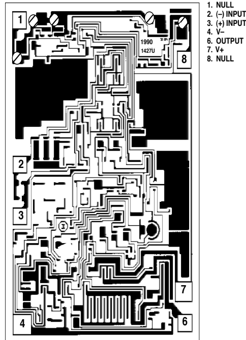
BINDING DIAGRAM
