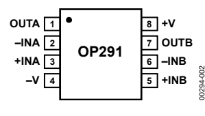
Figure 2. 8-Lead Narrow-Body SOIC
