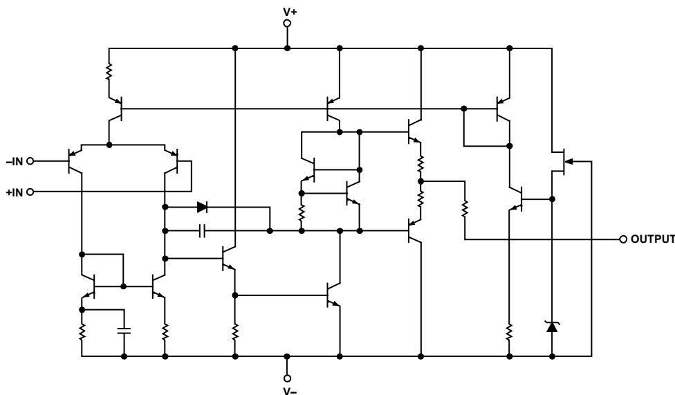
Figure 2. Simplified Schematic
