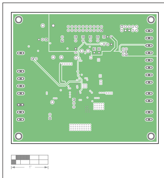
MAX25221 EV Kit PCB Layout—Internal Layer3
