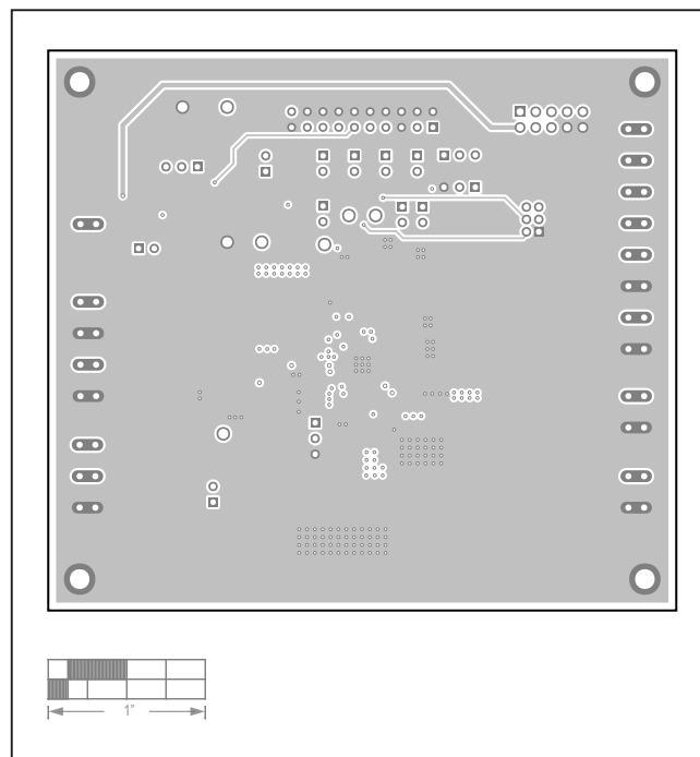
MAX25221 EV Kit PCB Layout—Internal Layer2
