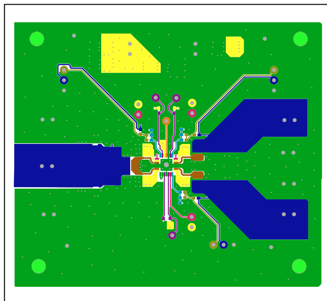
MAX20029B EV Kit PCB Layout—Top Layer
