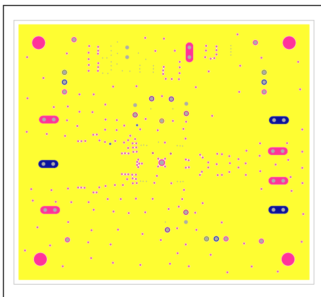
MAX20029B EV Kit PCB Layout—Inner Layer 2
