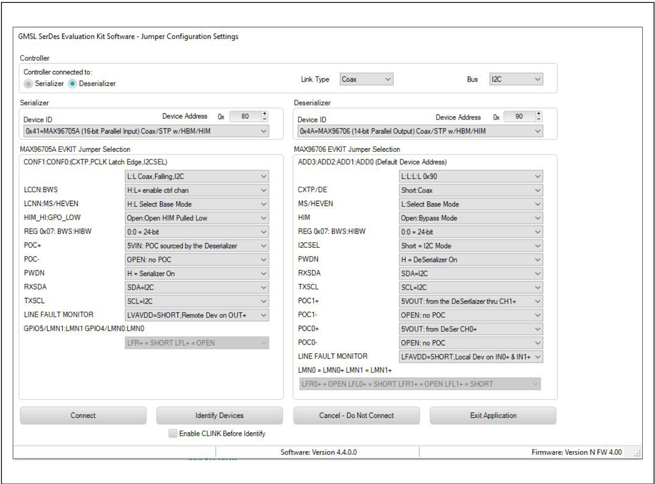
Figure 2. MAXSerDesEV-N EV Kit Software: Configuration Settings Window (shown with MAX96705A and MAX96706 EV Kits Connected)
