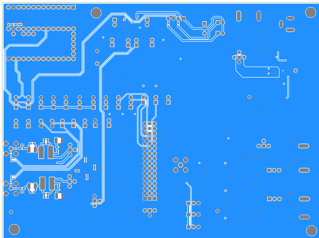
MAX96705A EV Kit PCB Layout—Bottom Layer
