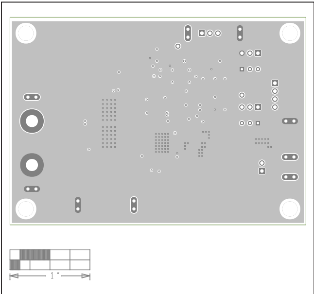
MAX25601 EV Kit PCB Layout—Internal2
