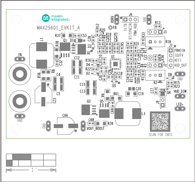
MAX25601 EV Kit Component Placement Guide—Top Silkscreen
