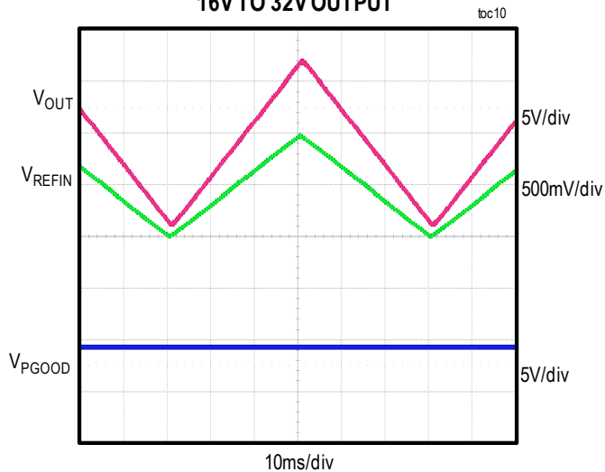
DYNAMIC REFIN RAMP RESPONSE 16V TO 32V OUTPUT
