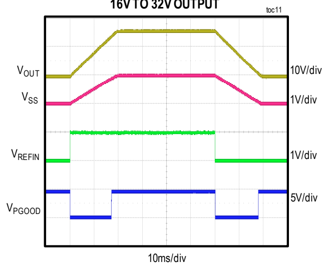
DYNAMIC REFIN STEP RESPONSE 16V TO 32V OUTPUT
