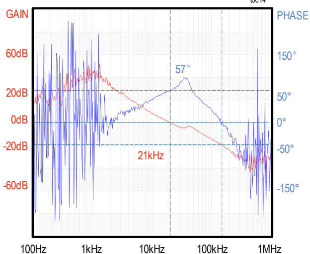
BODE PLOT 32V OUTPUT WITH 3A LOAD
