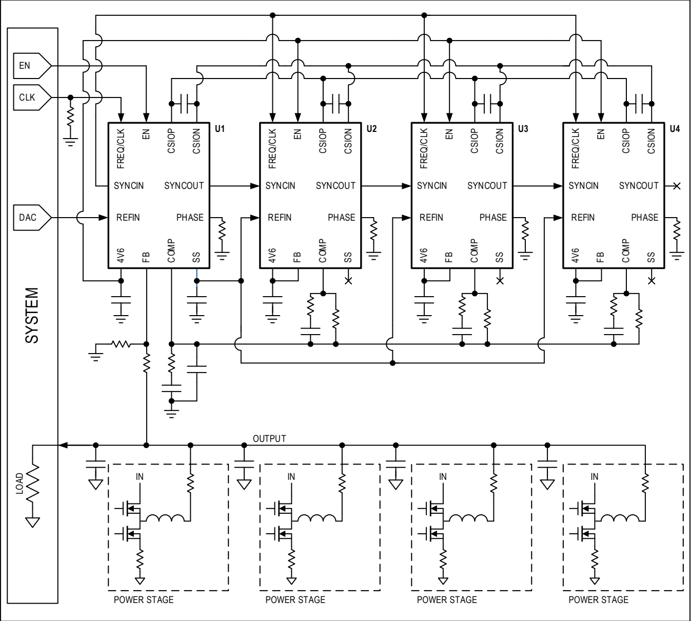
Figure 3. Multiphase Interconnects
