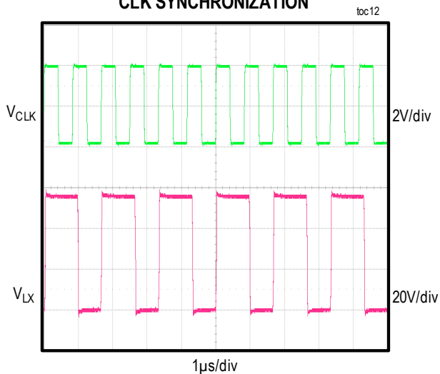
CLK SYNCHRONIZATION
