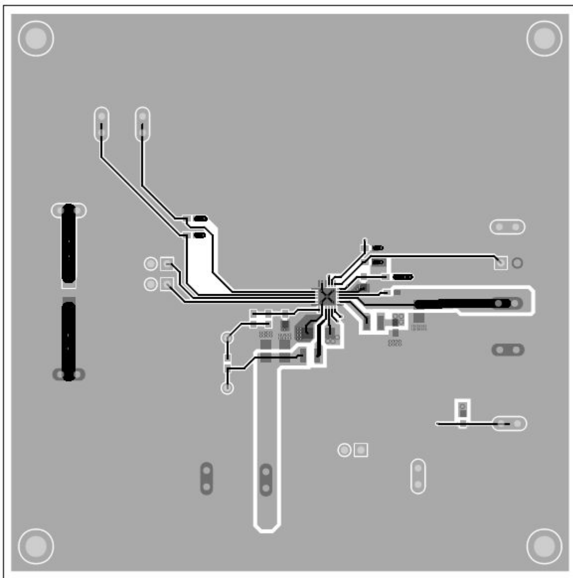
MAX20414 EV Kit Schematic PCB Layout—Top Layer
