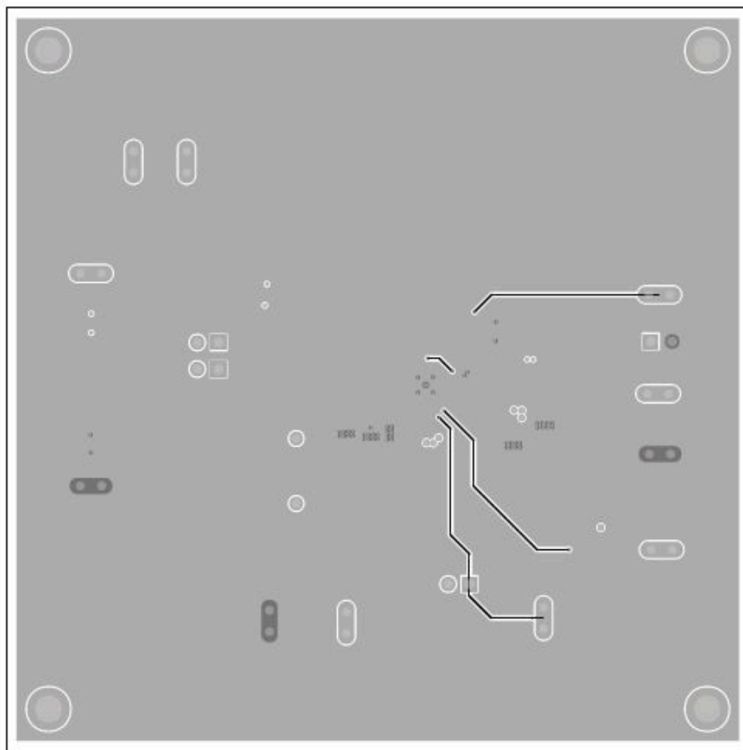
MAX20414 EV Kit Schematic PCB Layout—Bottom Layer
