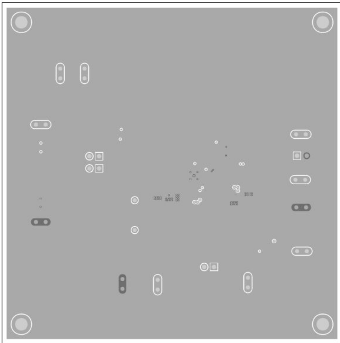
MAX20414 EV Kit Schematic PCB Layout—Internal Layer 2
