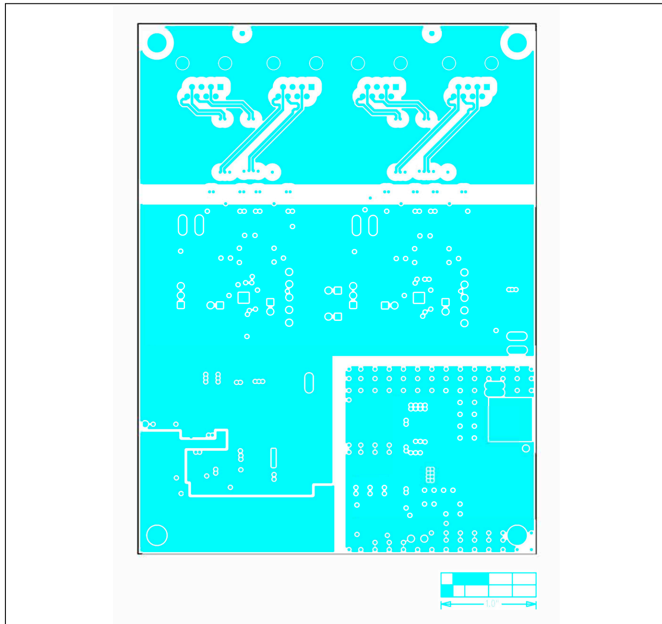
MAX5992 EV Kit—Layer 2 GND
