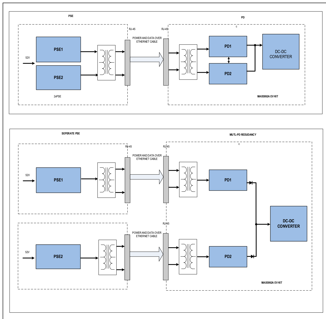
Figure 1. 2x2P Application, Multi-PD Redundancy
