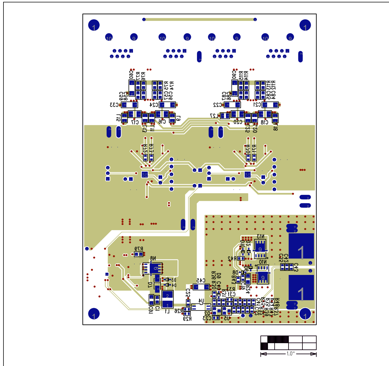
MAX5992 EV Kit—Bottom Layer
