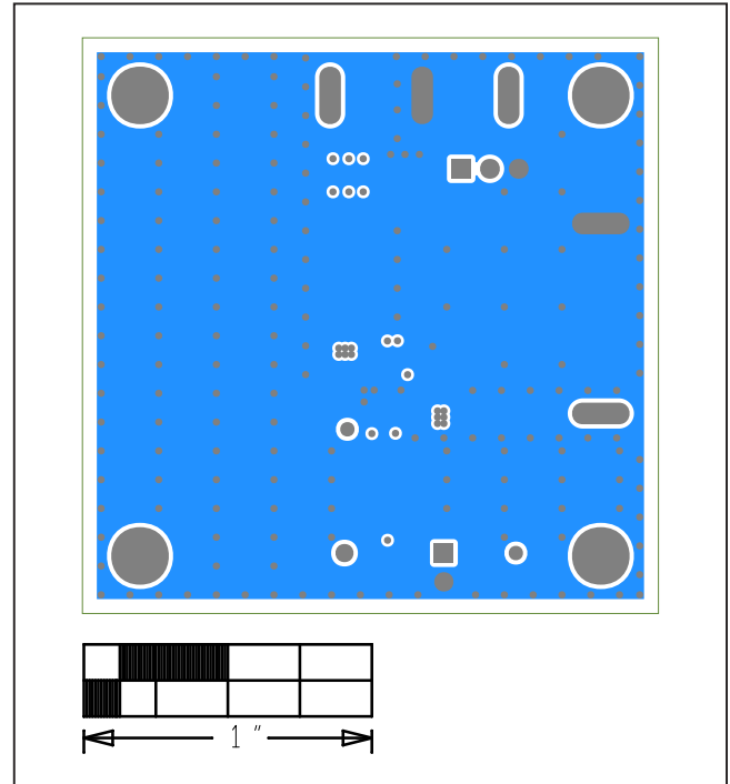
MAXM15463 EV Kit PCB Layout—Bottom Layer
