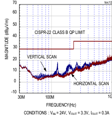
RADIATED EMISSION PLOT (C6 = 0.1μF, C7, C8, C9 = OPEN, L1 = SHORT)
