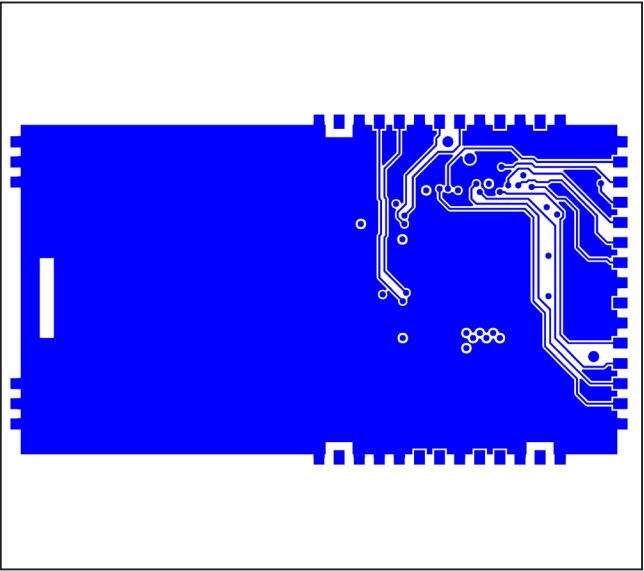
SC1905-DB3400—PCB Layout—Bottom
