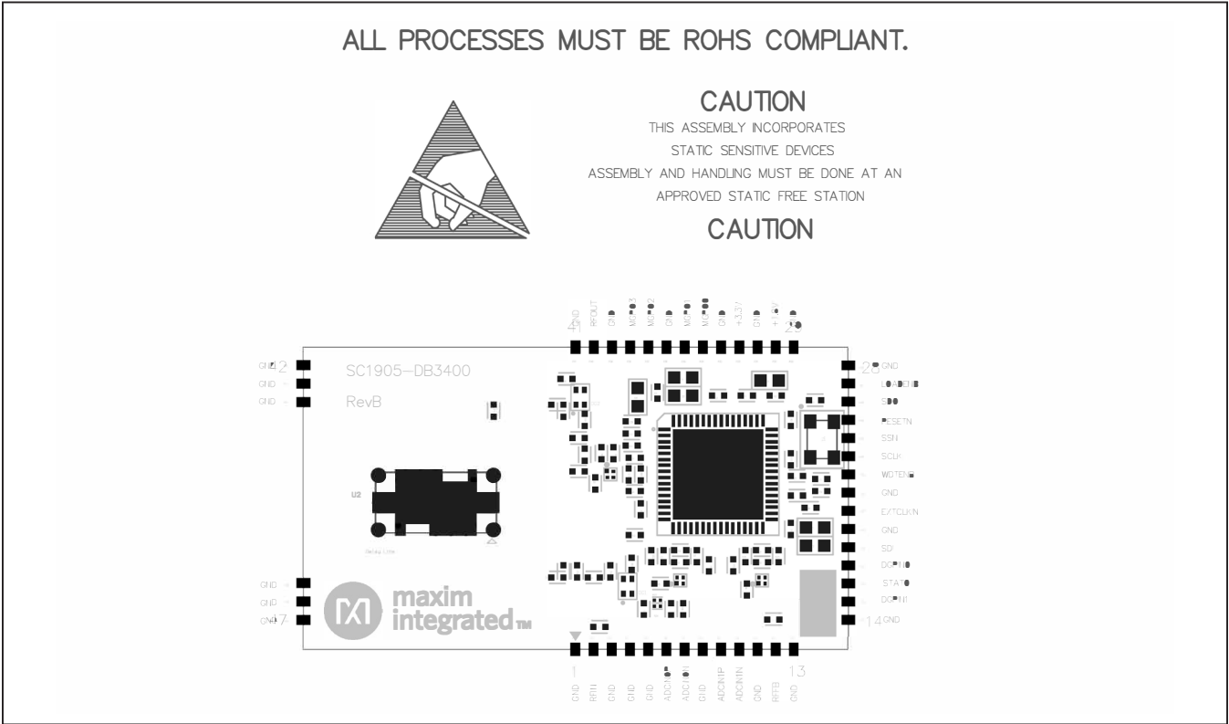
SC1905-DB3400—Assembly Drawing
