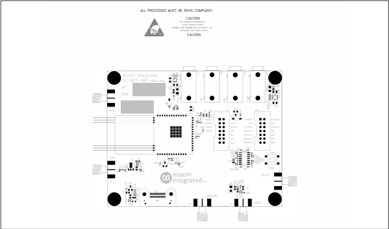
SC1905-MB—Assembly Drawing
