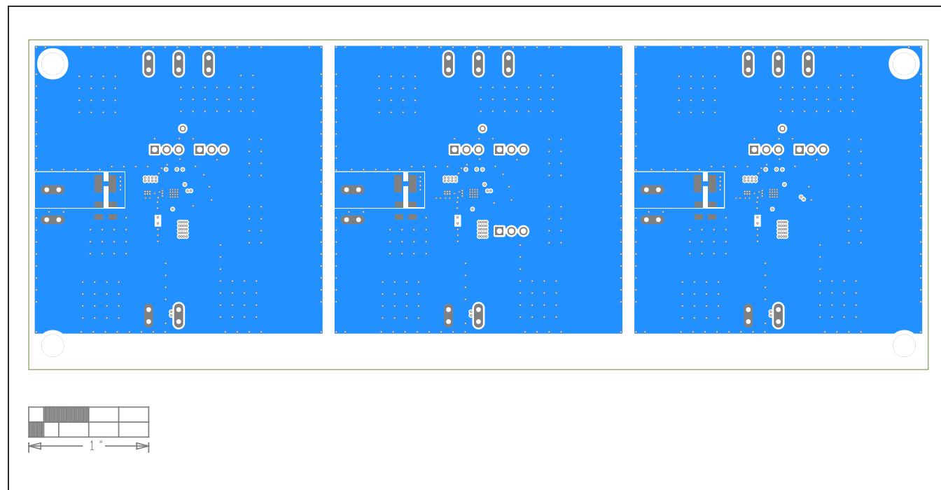
MAXM17633/MAXM17634/MAXM17635 EV Kits—Bottom Layer
