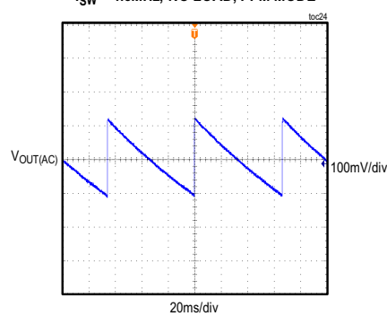
MAXM17635 STEADY-STATE OUTPUT-VOLTAGE RIPPLE V_{OUT} = 12V , f_{SW} = 1.8MHz , NO LOAD, PFM MODE
