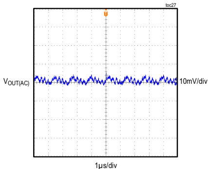
MAXM17635 STEADY-STATE OUTPUT-VOLTAGE RIPPLE V_{OUT} = 12V , f_{SW} = 1.8MHz , 20mA LOAD, DCM MODE
