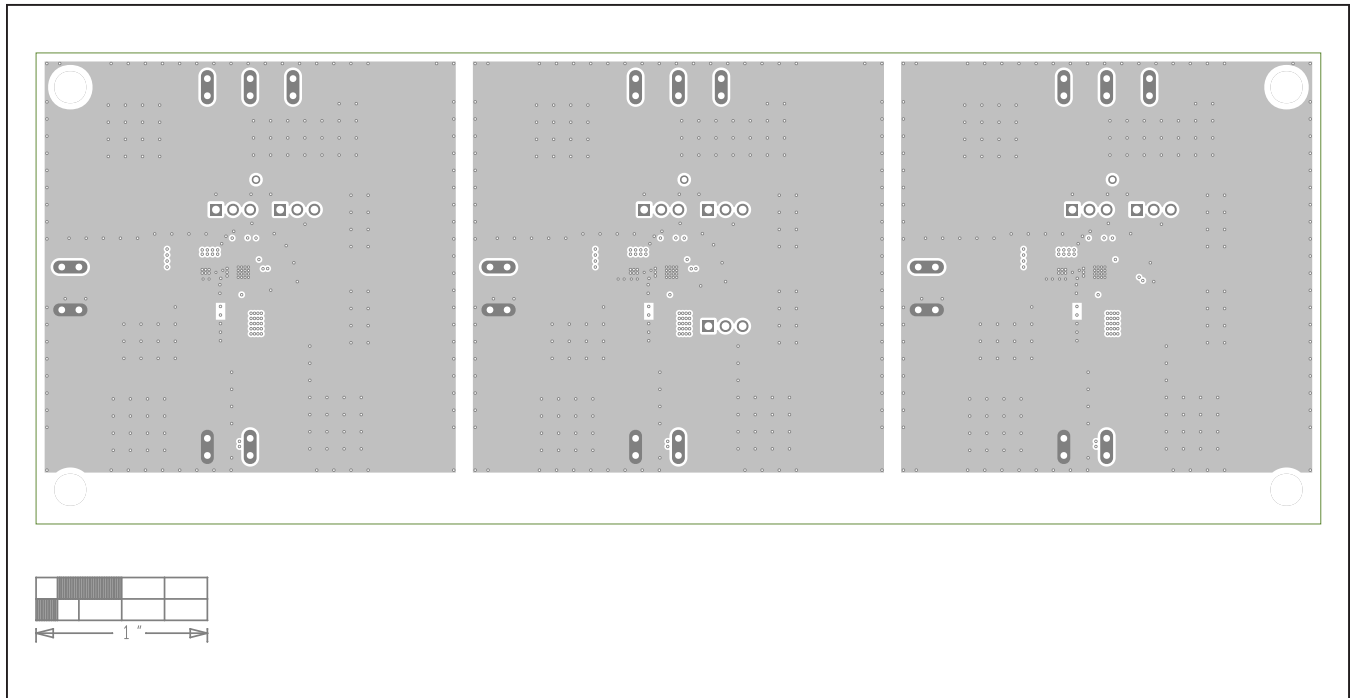
MAXM17633/MAXM17634/MAXM17635 EV Kits—Layer 2
