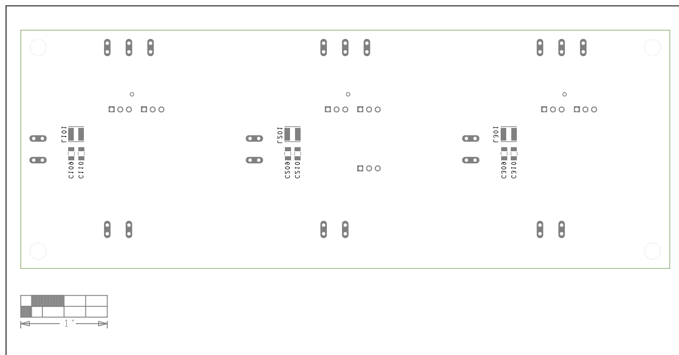
MAXM17633/MAXM17634/MAXM17635 EV Kits—Bottom Silkscreen
