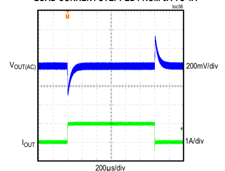
MAXM17635 LOAD-TRANSIENT RESPONSE V_{OUT} = 12V , f_{SW} = 1.8MHz , PWM MODE, LOAD CURRENT STEPPED FROM 0A TO 1A
