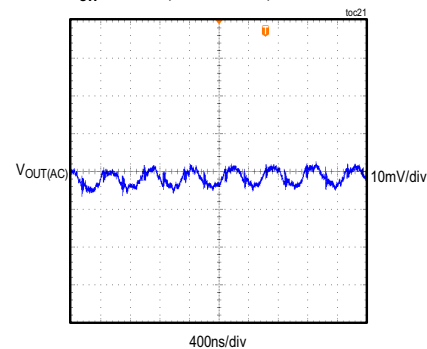
MAXM17635 STEADY-STATE OUTPUT-VOLTAGE RIPPLE V_{OUT} = 12V , f_{SW} = 1.8MHz , FULL LOAD, PWM MODE
