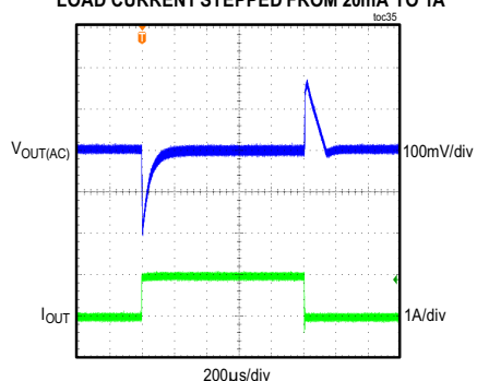
MAXM17634 LOAD-TRANSIENT RESPONSE V_{OUT} = 5V , f_{SW} = 1MHz , DCM MODE, LOAD CURRENT STEPPED FROM 20mA TO 1A
